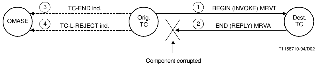
FIGURE 2b/Q.754
