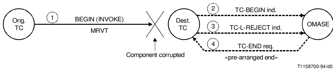
FIGURE 2a/Q.754
