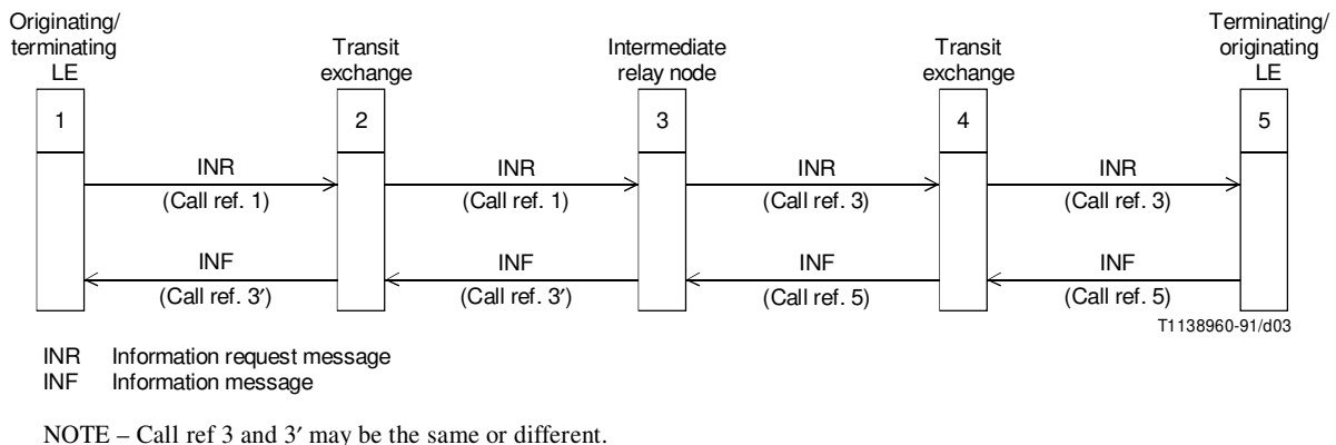
FIGURE 3/Q.730
