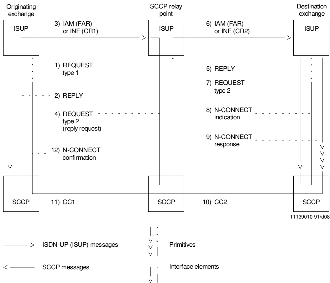
FIGURE 8/Q.730
