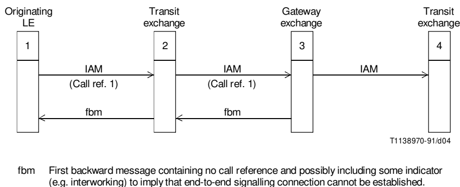
FIGURE 4/Q.730
