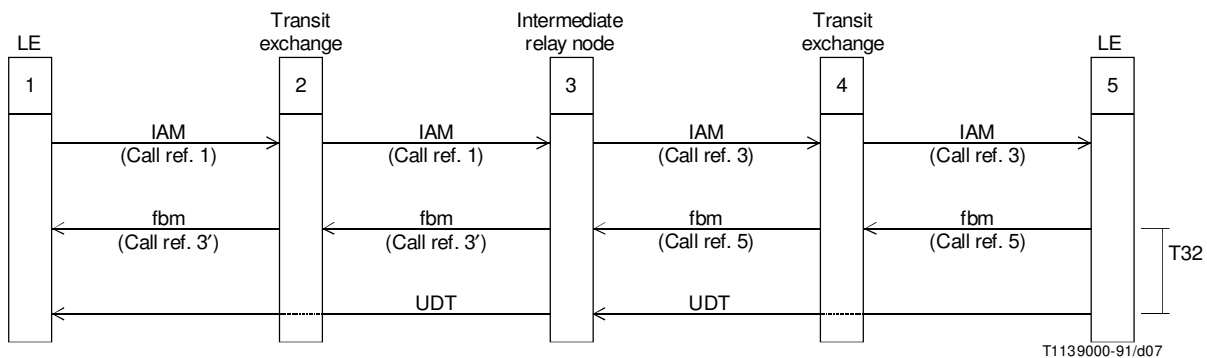
FIGURE 7/Q.730
