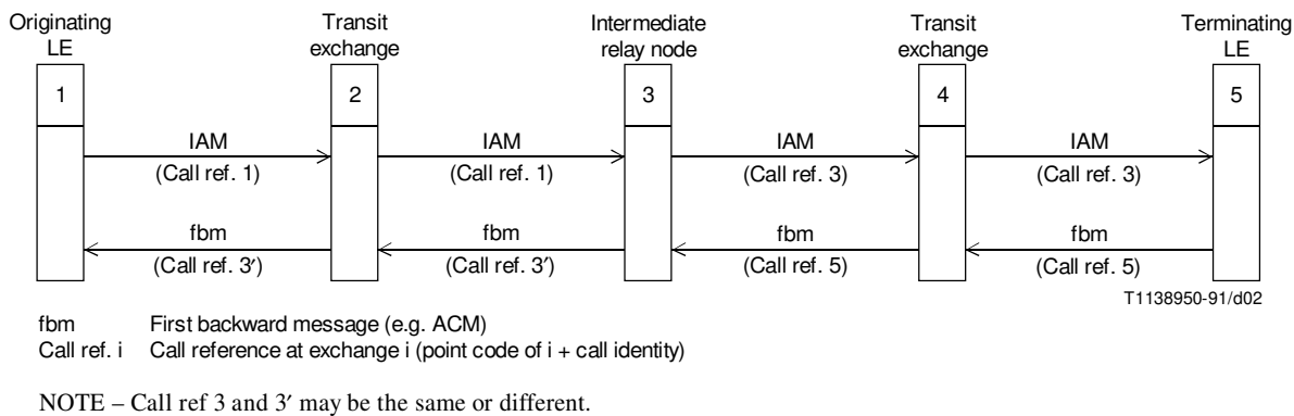
FIGURE 2/Q.730
