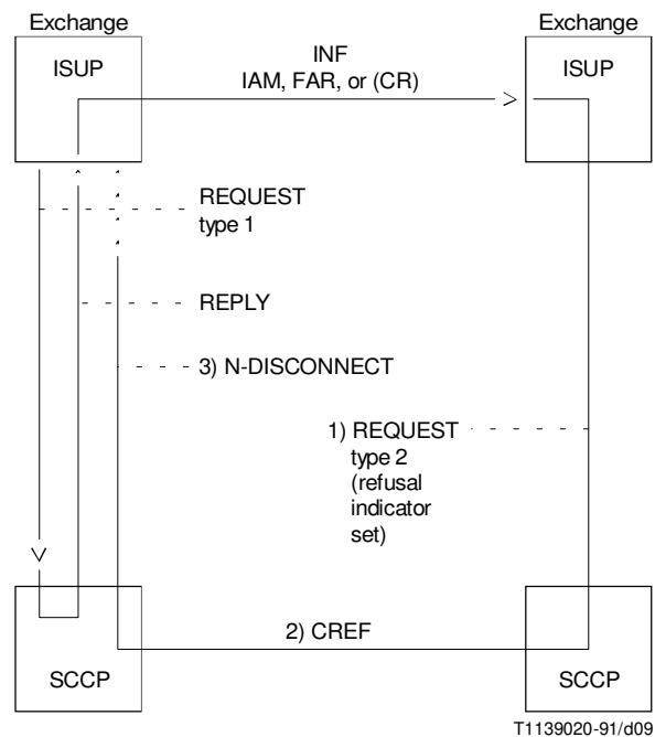
FIGURE 9/Q.730
