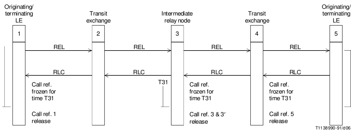
FIGURE 6/Q.730 Simultaneous release of a bearer connection and ISDN user part end-to-end signalling connection based on connectionless class
