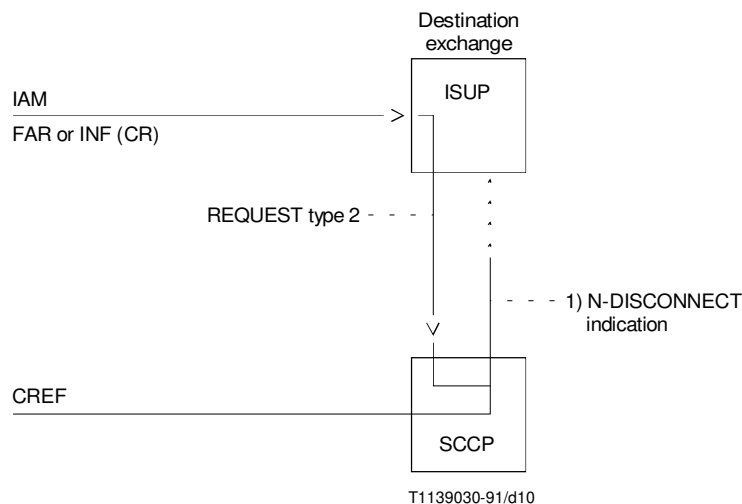
FIGURE 10/Q.730
