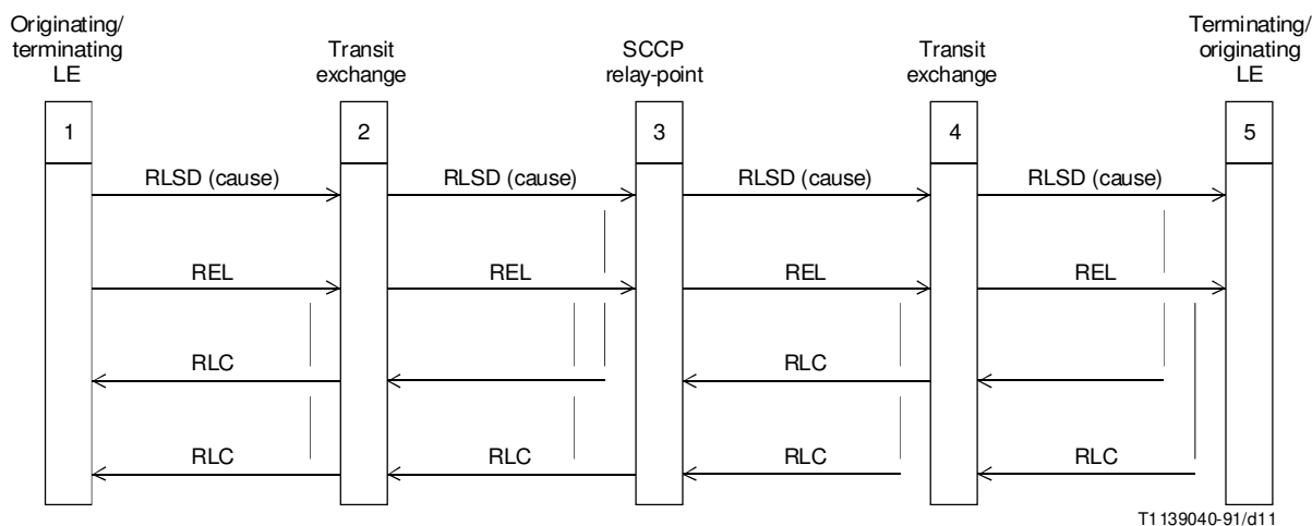
FIGURE 11/Q.730
