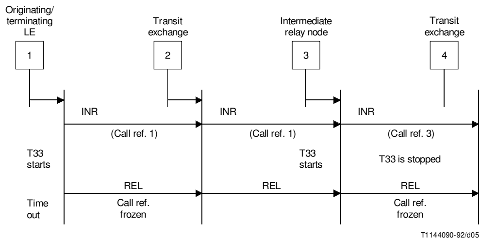
FIGURE 5/Q.730 No response from SCCP after time T33 after the transmission of the originating call reference, during the establishment of an ISDN user part end-to-end signalling connection based on SCCP connectionless class
