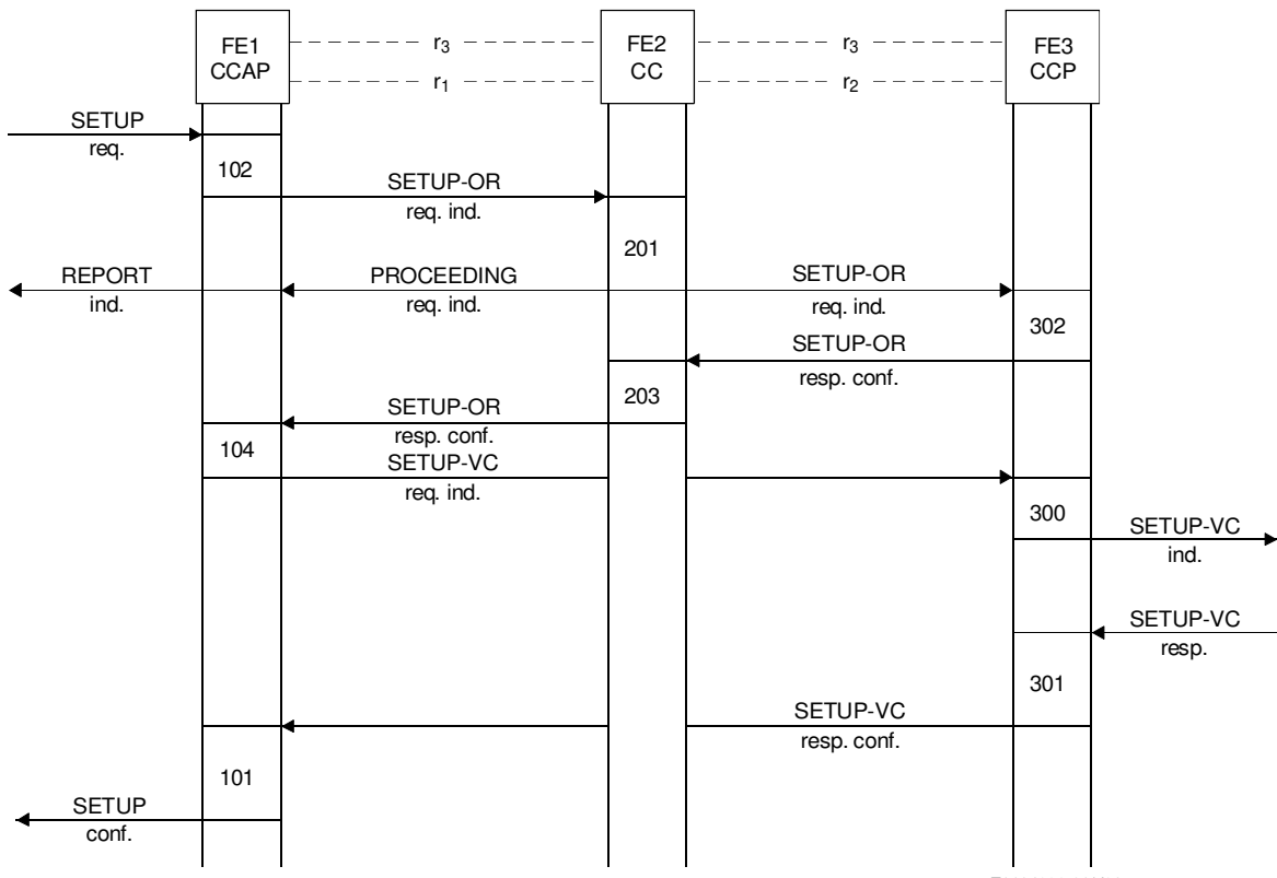
FIGURE 1-3/Q.72 Originating access situation, B-channel required (OAS2)
