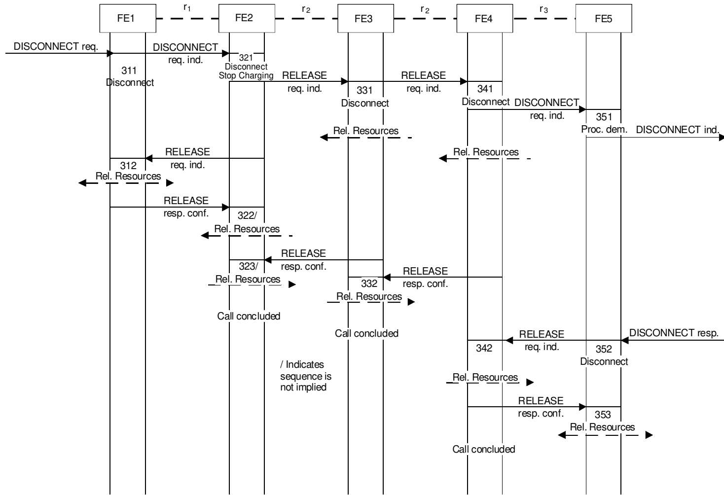
FIGURE 2-3/Q.72 Normal clearing – frame mode call calling party disconnect
