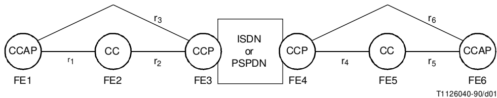
FIGURE 1-1/Q.72 Functional model
