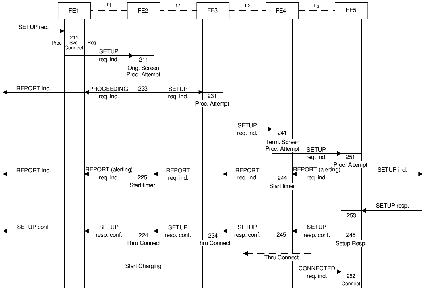
FIGURE 2-2/Q.72 Successful frame mode call set-up
