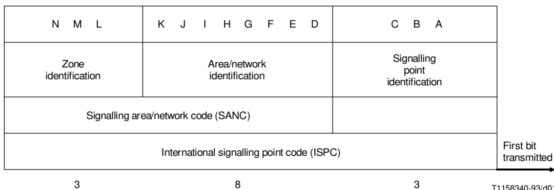
FIGURE 1/Q.708 Format for international signalling point code (ISPC)
