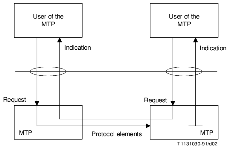
FIGURE 2/Q.701 Specific name of primitives and peer-to-peer communications
