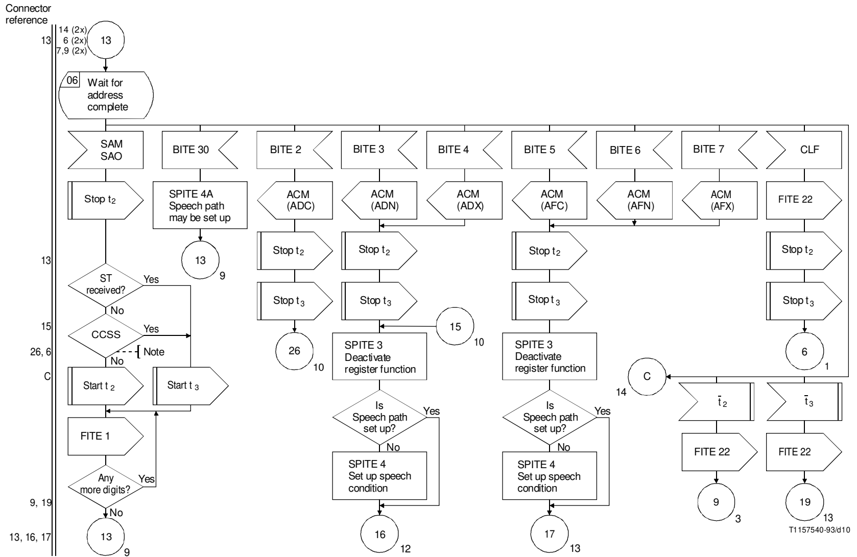
FIGURE 3/Q.614 (sheet 9 of 14) Incoming Signalling System No. 7 (TUP)
