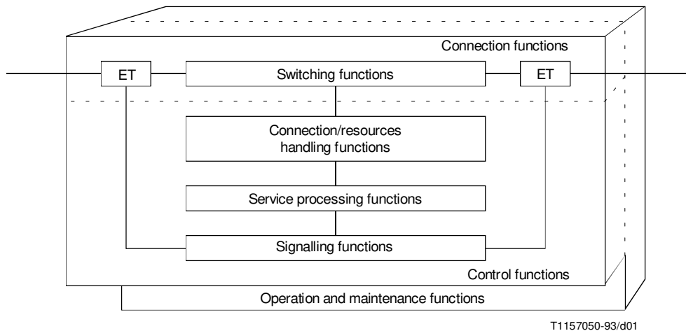
FIGURE 1/Q.521 Exchange functional model
