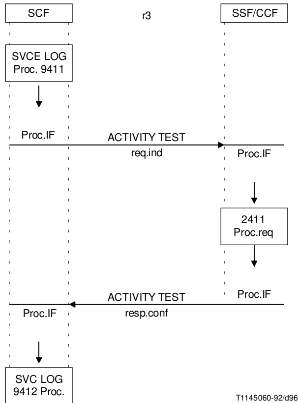
FIGURE 5-63/Q.1214 Information flow diagram activity test functionality
