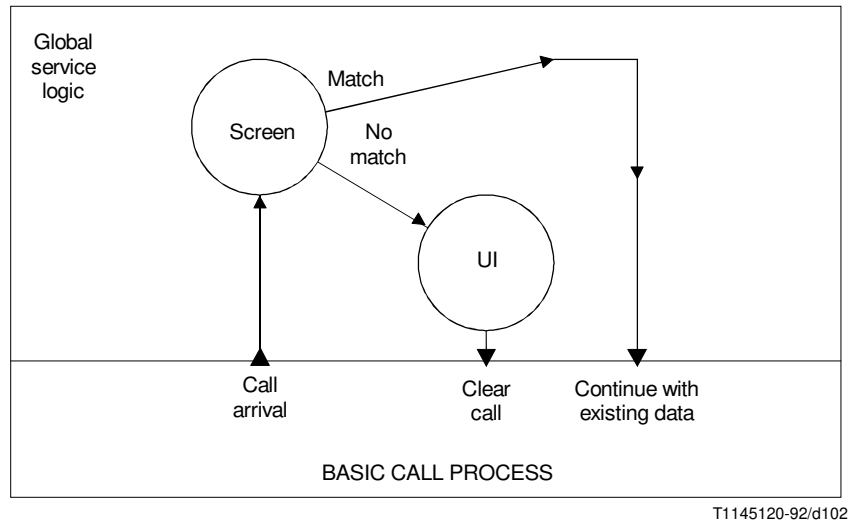
FIGURE 5-69/Q.1214 GFP terminating screening service
