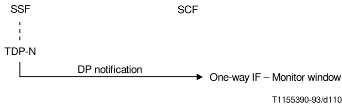
FIGURE B.2/Q.1214 (sheet 1 of 12) SSF/CCF - SCF relationship scenarios
