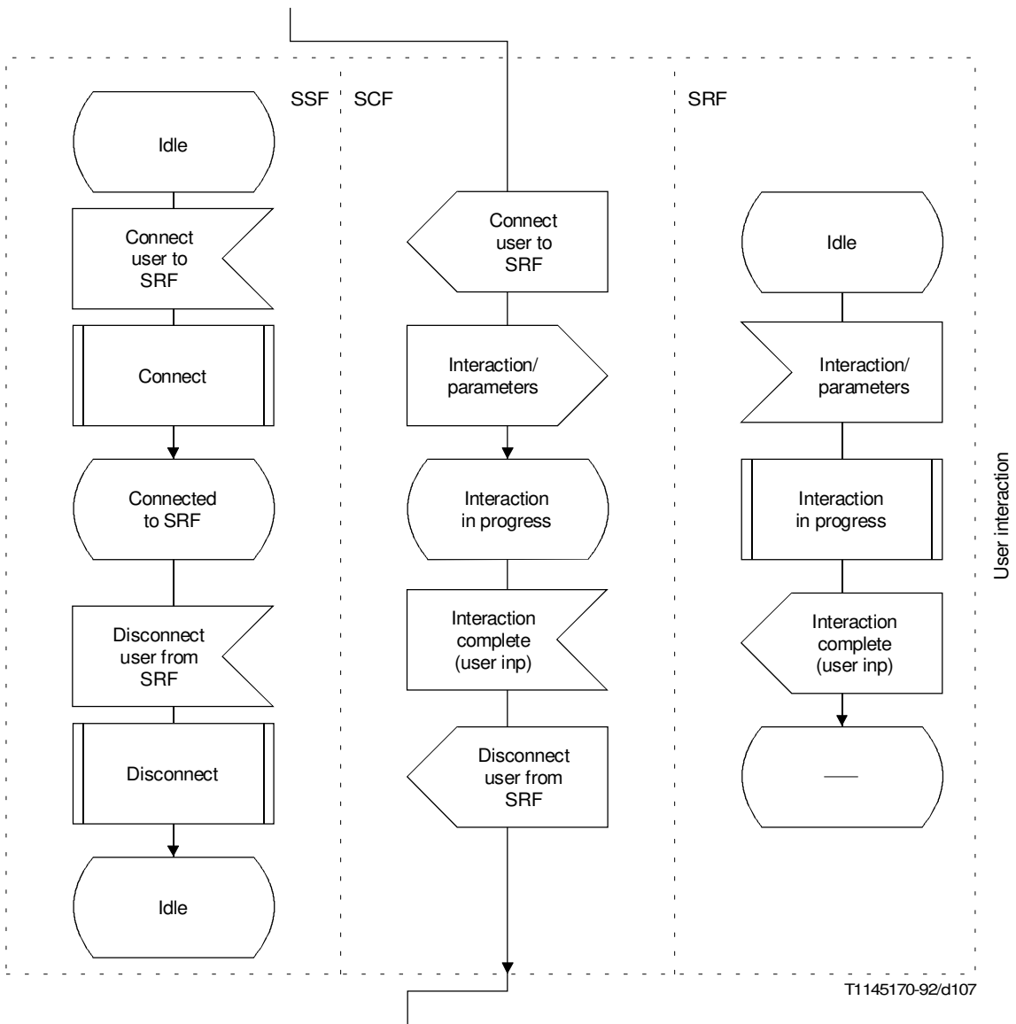
FIGURE 5-70/Q.1214 (sheet 5 of 5) DFP terminating screening showing DFP SIB representations
