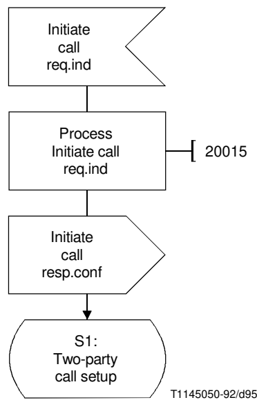
FIGURE 5-62/Q.1214 SDL diagram “basic call process” SIB (call initiation)
