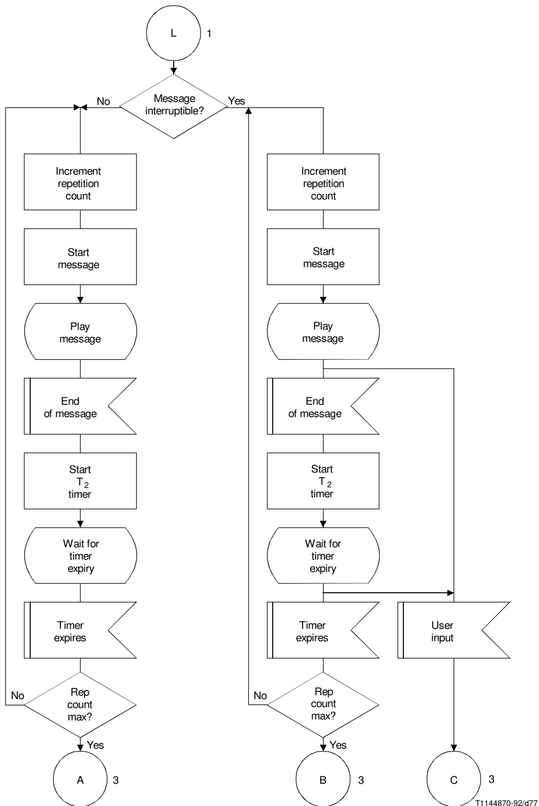
FIGURE 5-49/Q.1214 (sheet 2 de 5)
