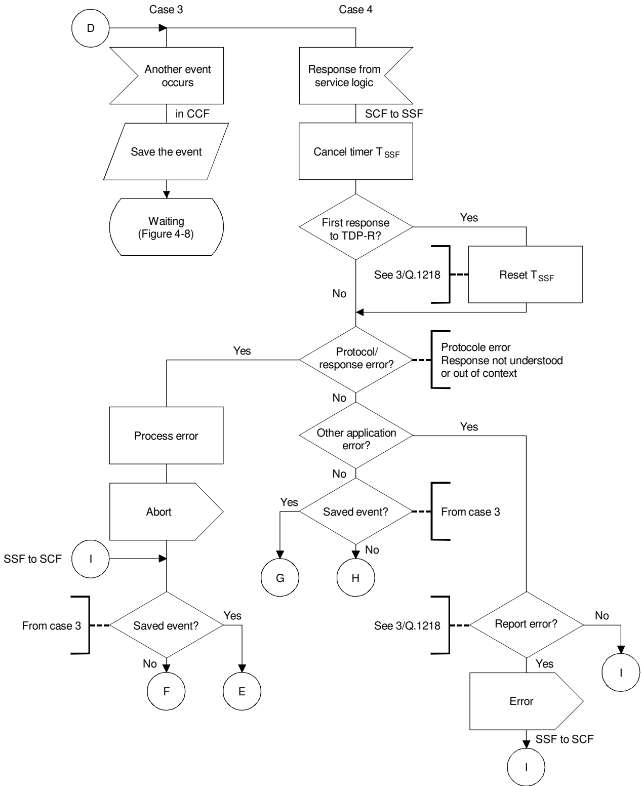
FIGURE 4-9/Q.1214 Detection point processing
