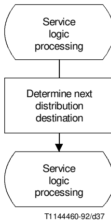
FIGURE 5-13/Q.1214 Stage 2 – distribution SIB
