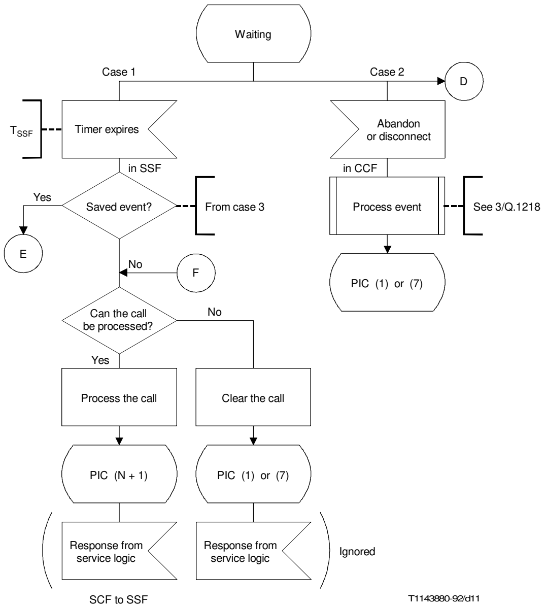
FIGURE 4-8/Q.1214 Detection point processing
