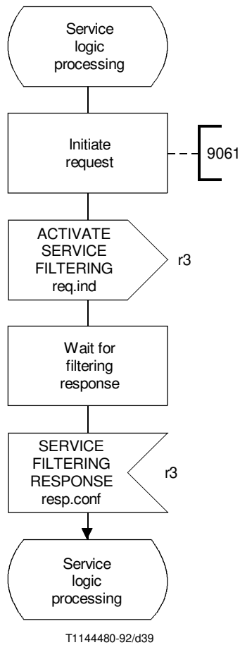
FIGURE 5-15/Q.1214 SCF actions for the “limit” SIB
