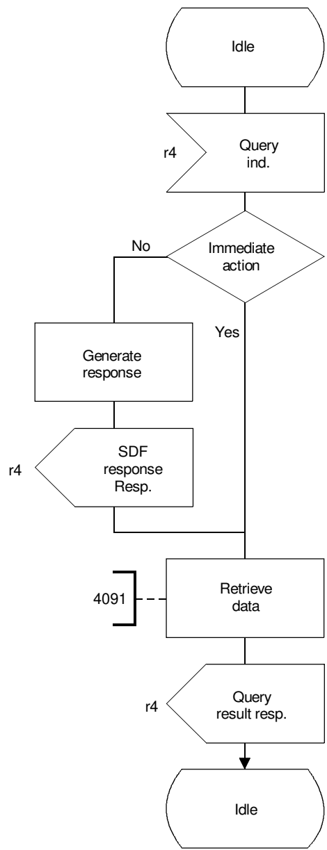
FIGURE 5-34/Q.1214 “Service data management” SIB service data functional entity
