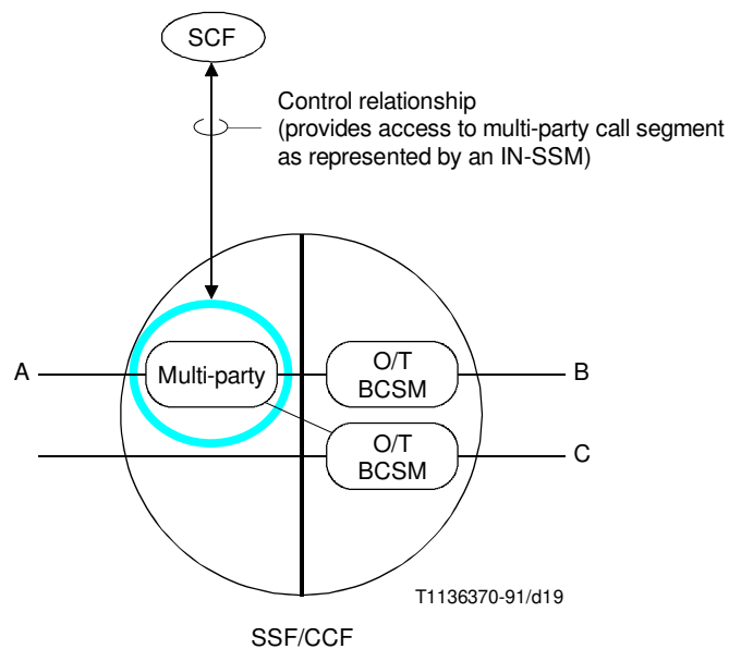
FIGURE 4-16/Q.1214 Single-ended control of a multi-party call
