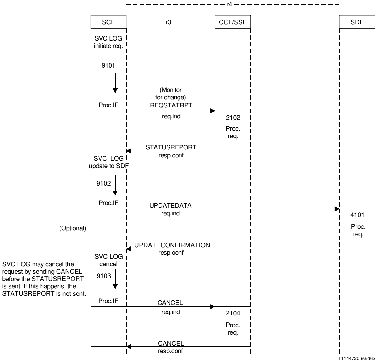
FIGURE 5-38/Q.1214 Information flow diagram “status notification” SIB
