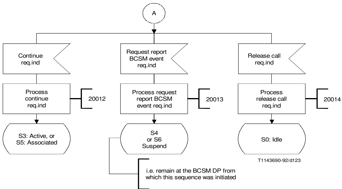
FIGURE I.2/Q.1214 “Basic call process” SIB (continuation of active)
