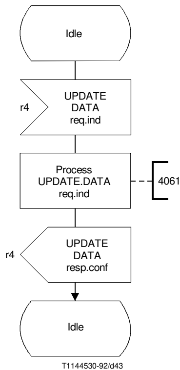
FIGURE 5-20/Q.1214 SDF actions for the “log call information” SIB
