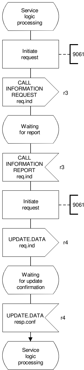
FIGURE 5-18/Q.1214 SCF actions for the “log call information” SIB
