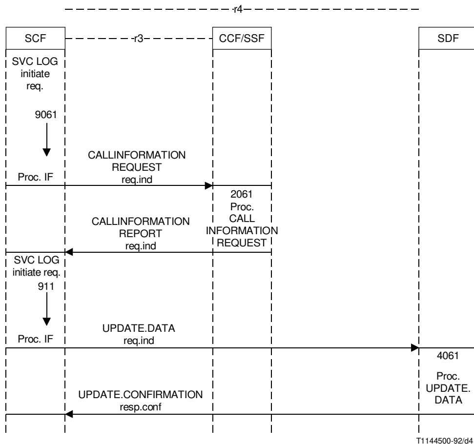
FIGURE 5-17/Q.1214 Information flow diagram “log call information” SIB
