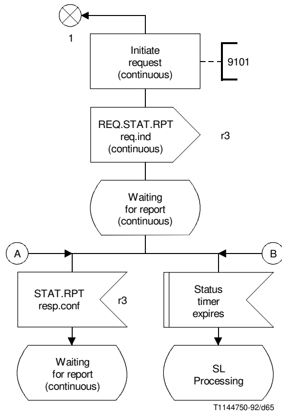
FIGURE 5-40/Q.1214 (sheet 2 of 2) “Status notification” SIB SCF
