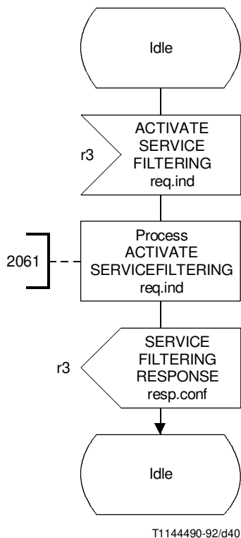
FIGURE 5-16/Q.1214 CCF/SSF actions for the “limit” SIB
