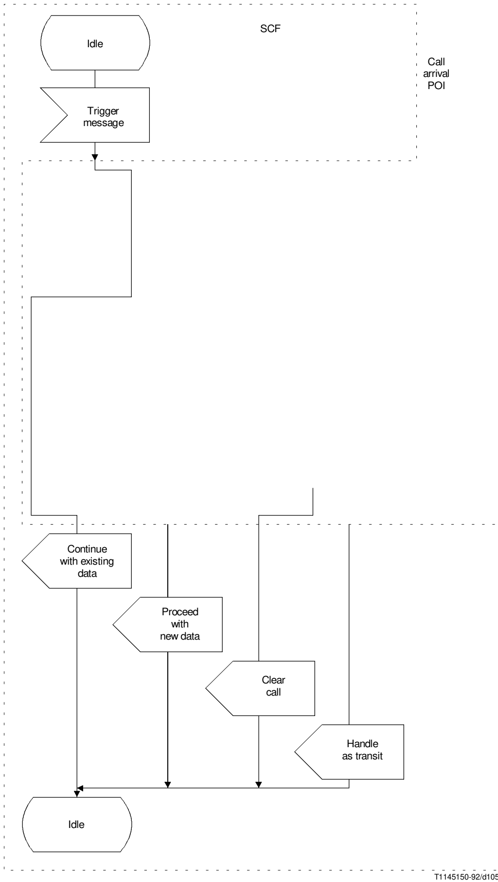
FIGURE 5-70/Q.1214 (sheet 3 of 5) DFP terminating screening showing DFP SIB representations
