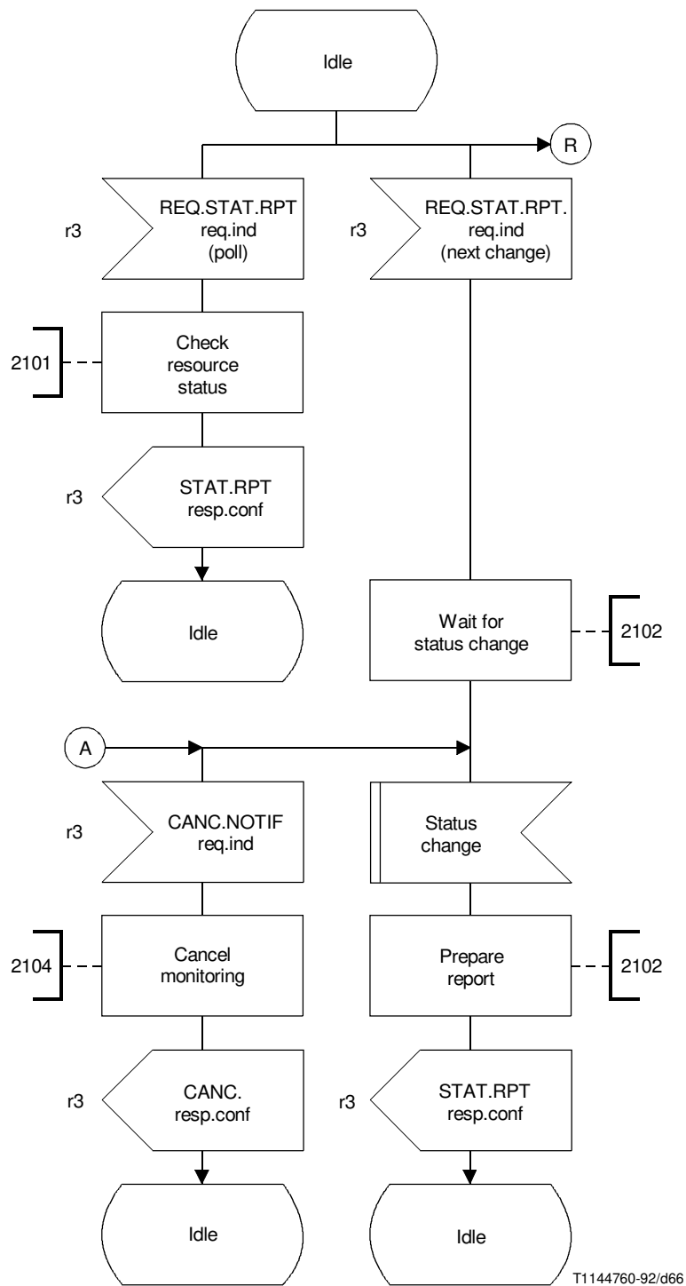
FIGURE 5-41/Q.1214 (sheet 1 of 2)
