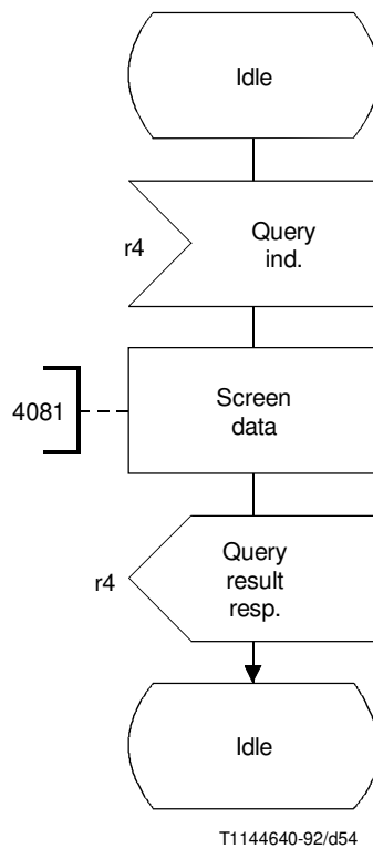
FIGURE 5-30/Q.1214 “Screen” SIB service data functional entity
