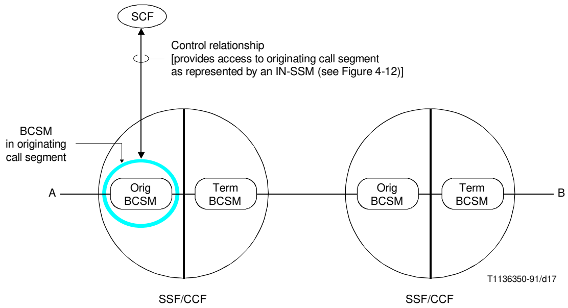
FIGURE 4-14/Q.1214 Single-ended control of a two-party call
