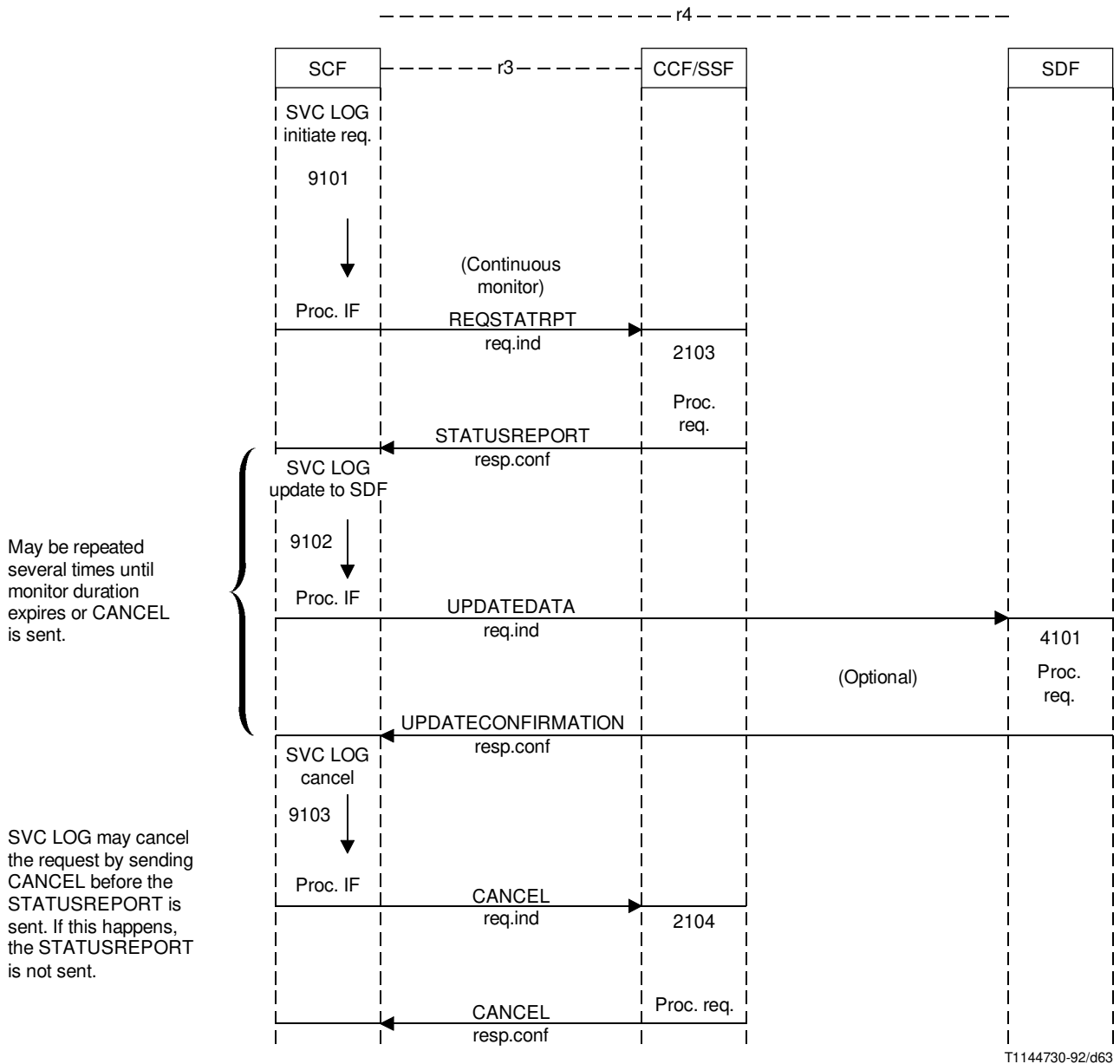
FIGURE 5-39/Q.1214 Information flow diagram “status notification” SIB
