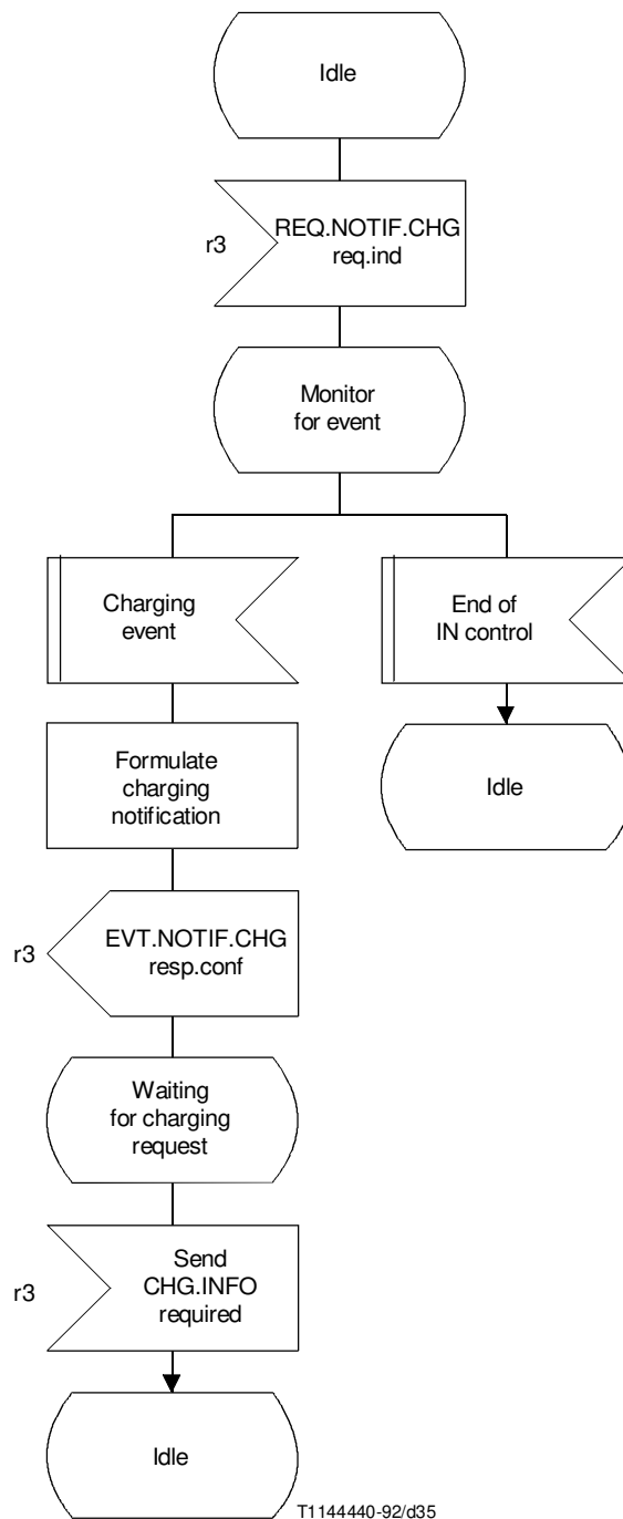
FIGURE 5-11/Q.1214 CCF/SSF-charging event “charge” SIB
