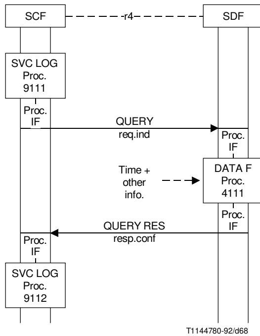
FIGURE 5-42/Q.1214 Information flow diagram “translate” SIB
