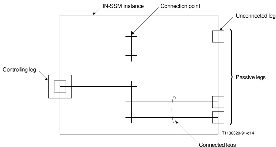
FIGURE 4-11/Q.1214 Connection control IN-SSM instance
