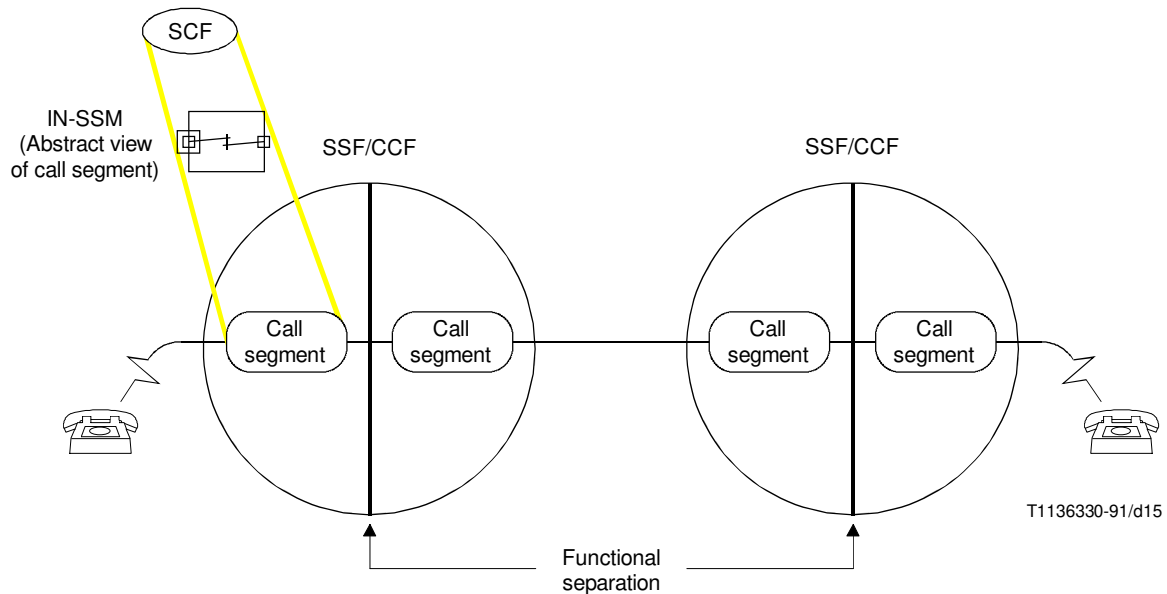
FIGURE 4-12/Q.1214 Call segments in two-party inter-SSF/CCF call
