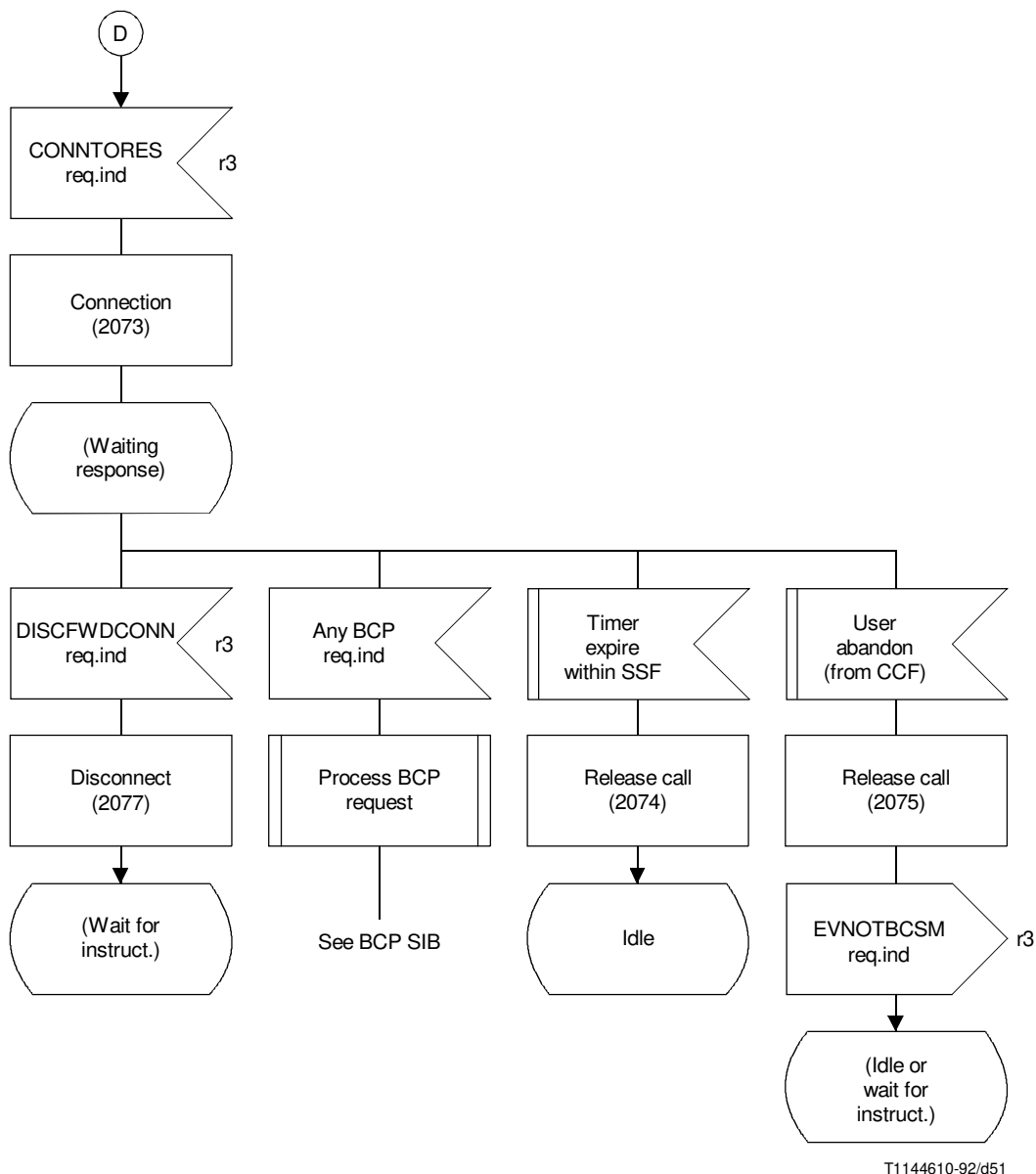
FIGURE 5-27/Q.1214 SSF actions for “queue” SIB
