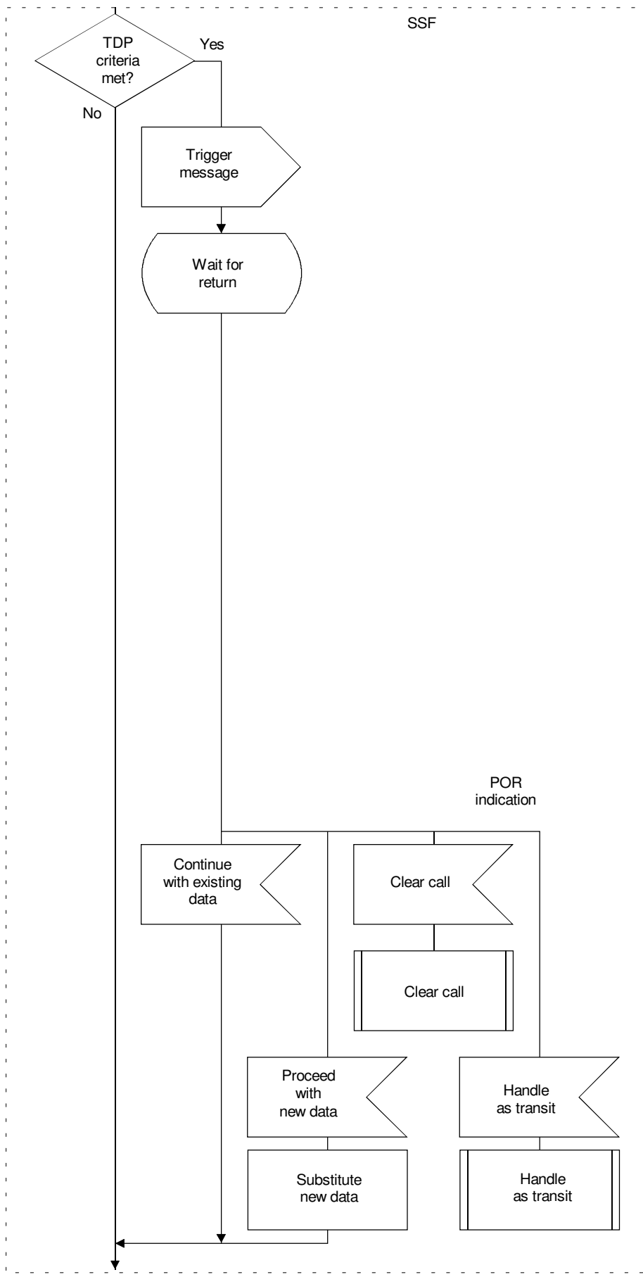
FIGURE 5-70/Q.1214 (sheet 2 of 5) DFP terminating screening showing DFP SIB representations
