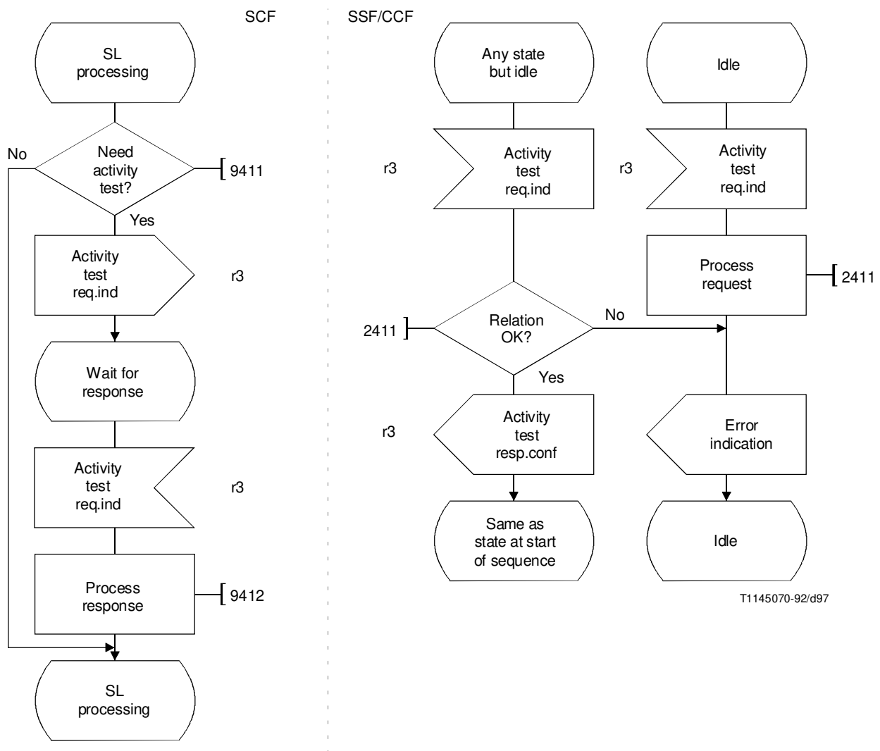
FIGURE 5-64/Q.1214 SDLs for activity test
