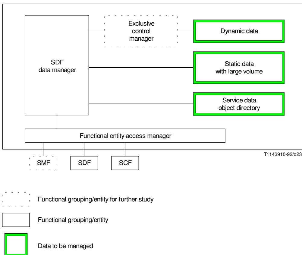
FIGURE 4-20/Q.1214 SDF model
