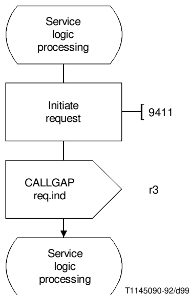
FIGURE 5-66/Q.1214 SCF actions for the call gap capability
