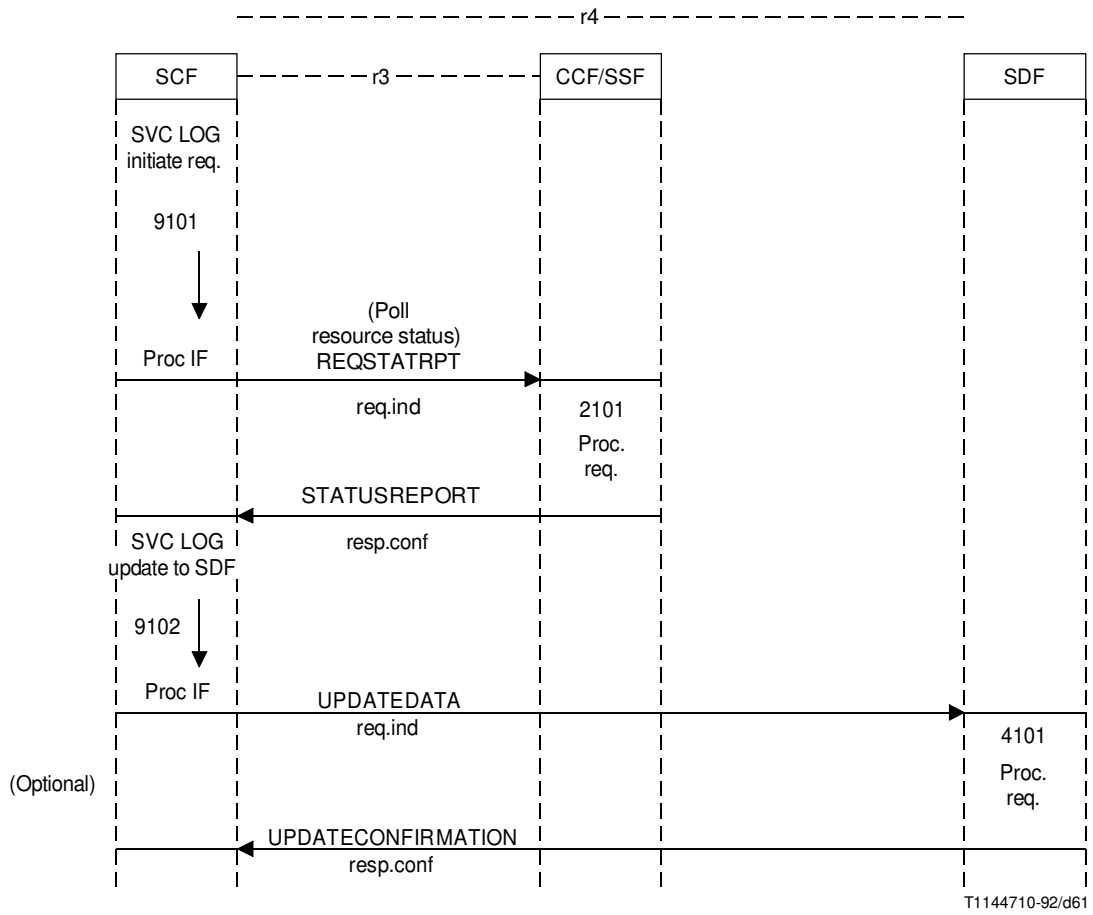
FIGURE 5-37/Q.1214 Information flow diagram “status notification” SIB
