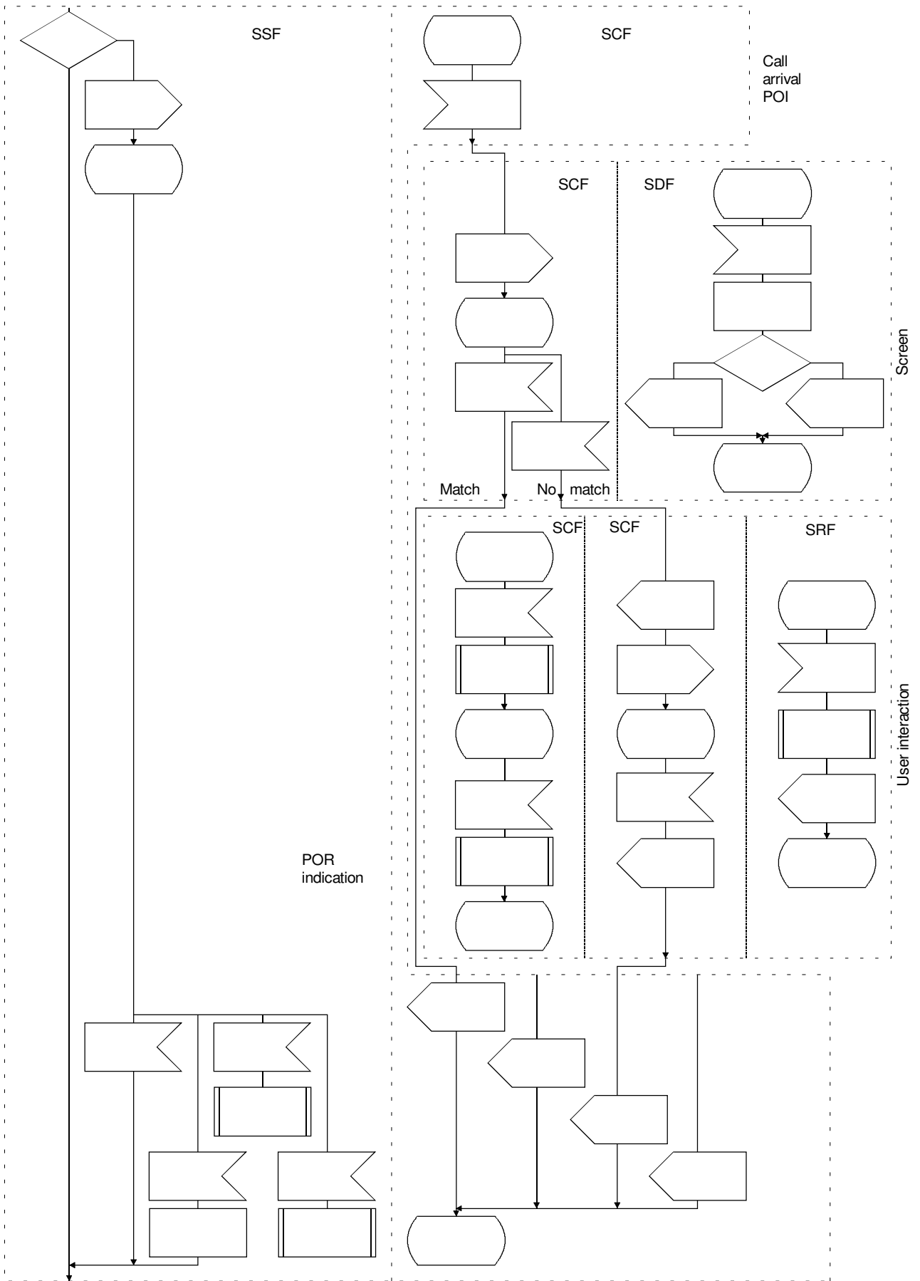
FIGURE 5-70/Q.1214 (sheet 1 of 5)
