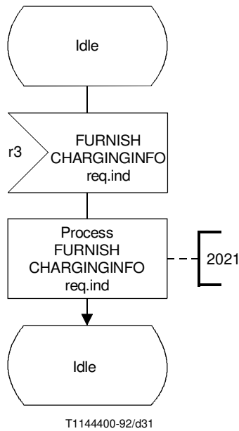
FIGURE 5-7/Q.1214 CCF/SSF actions for the “charge” SIB, Type 1
