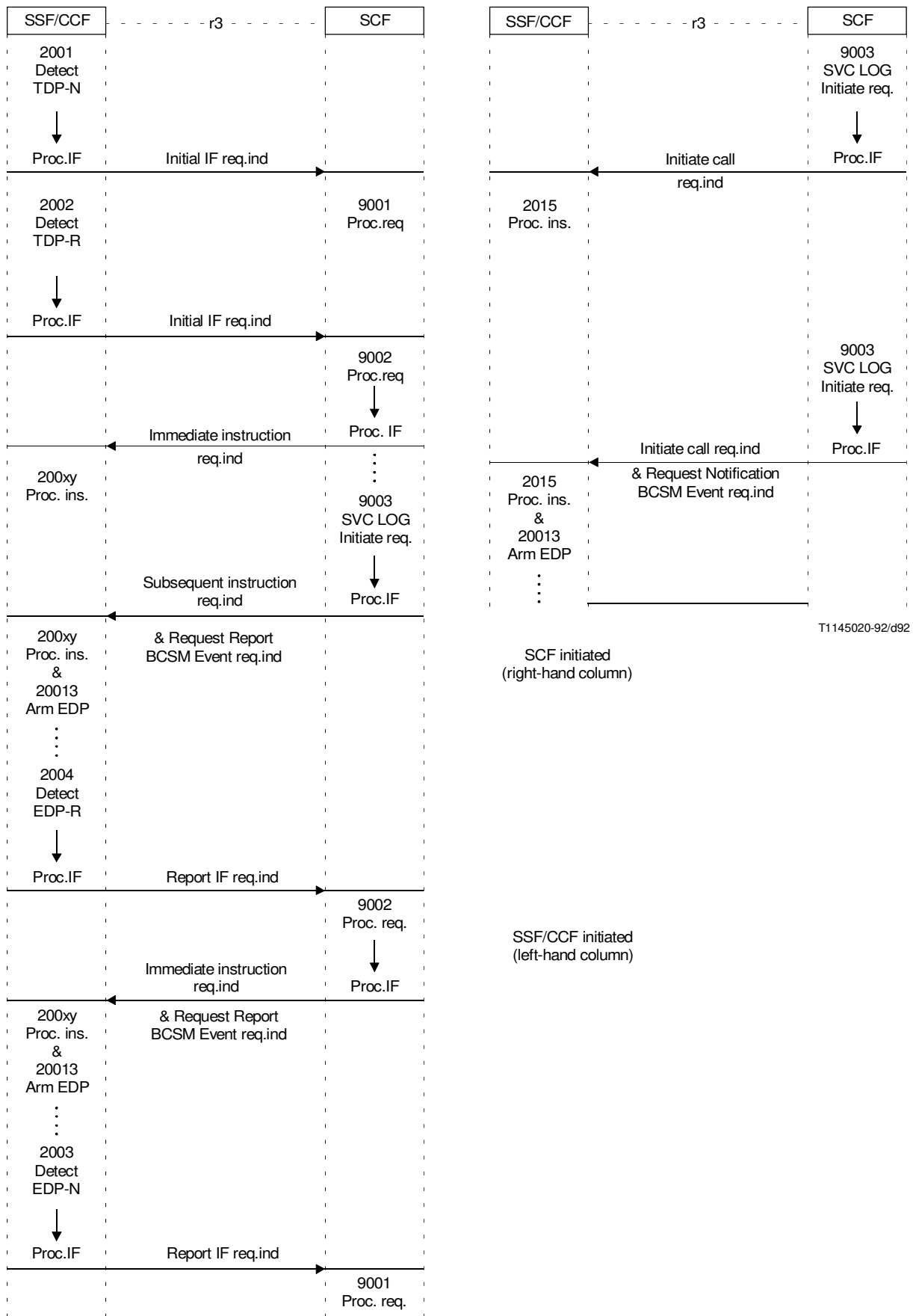
FIGURE 5-59/Q.1214 Information flow diagram basic call process SIB
