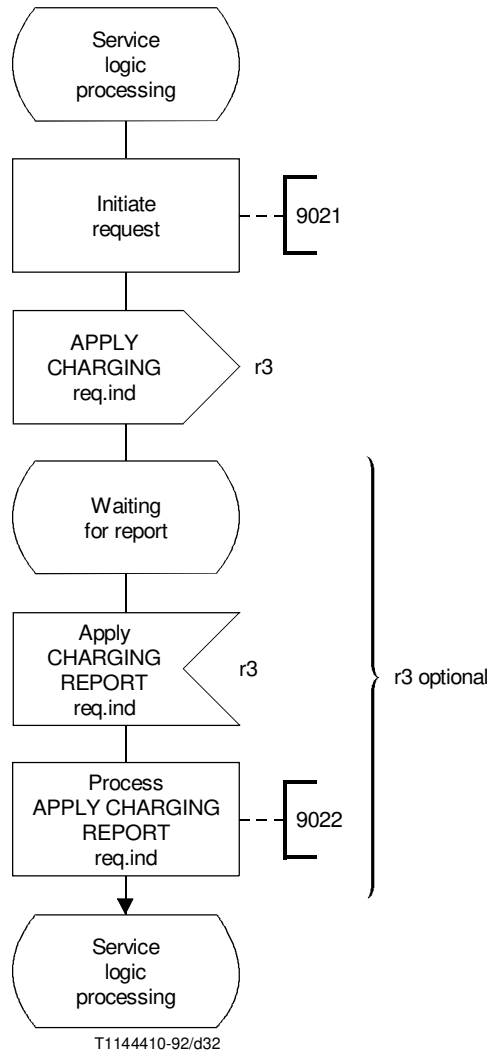
FIGURE 5-8/Q.1214 SCF actions for the “charge” SIB
