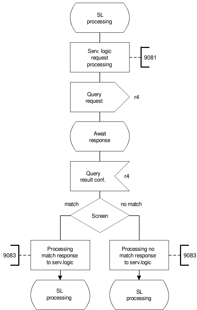
FIGURE 5-29/Q.1214 “Screen” SIB service control functional entity
