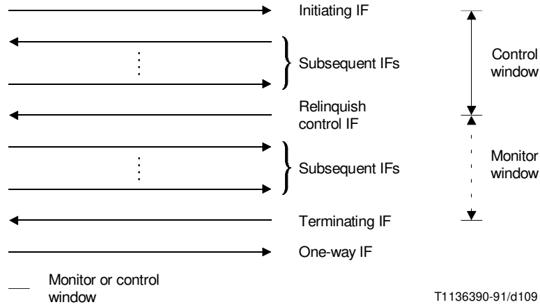
FIGURE B.1/Q.1214 General information flow terminology
