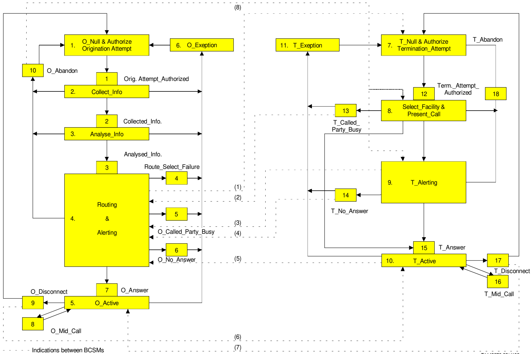
FIGURE A.1/Q.1214 BCSM indications
