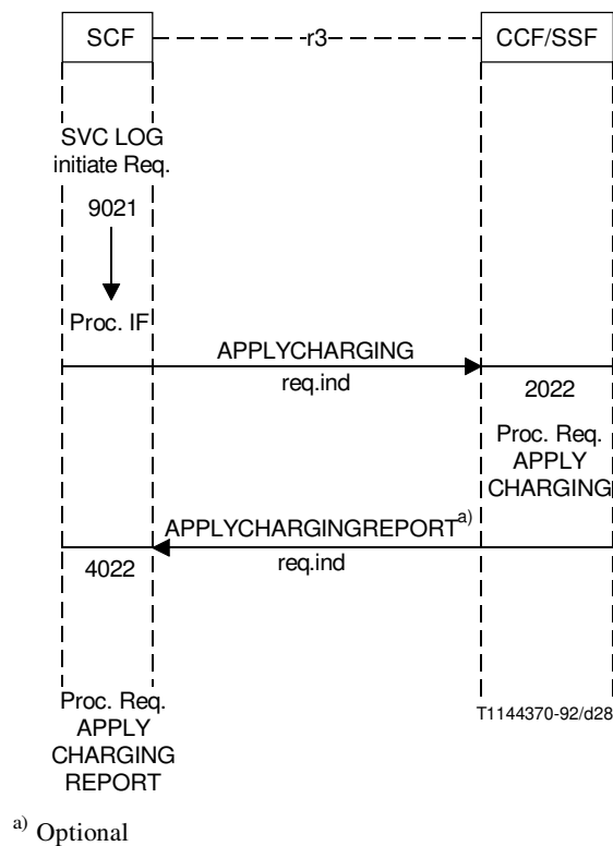
FIGURE 5-4/Q.1214 Information flow diagram “charge” SIB Type 2
