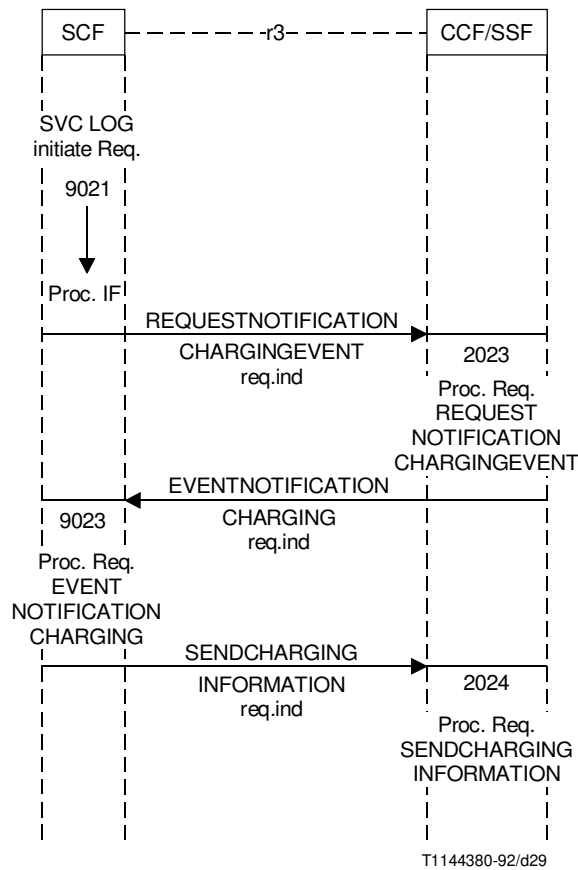
FIGURE 5-5/Q.1214 Information flow diagram “charge” SIB Type 3
