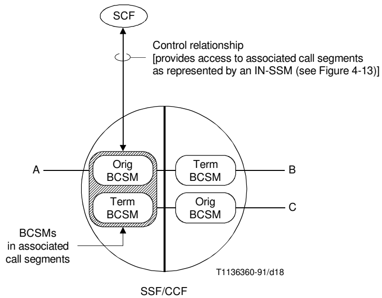
FIGURE 4-15/Q.1214 Single-ended control of associated calls
