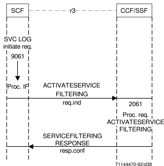
FIGURE 5-14/Q.1214 Information flow diagram “limit” SIB
