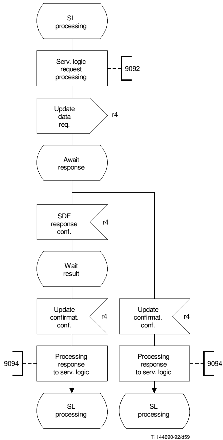
FIGURE 5-35/Q.1214 “Service data management” SIB service control functional entity
