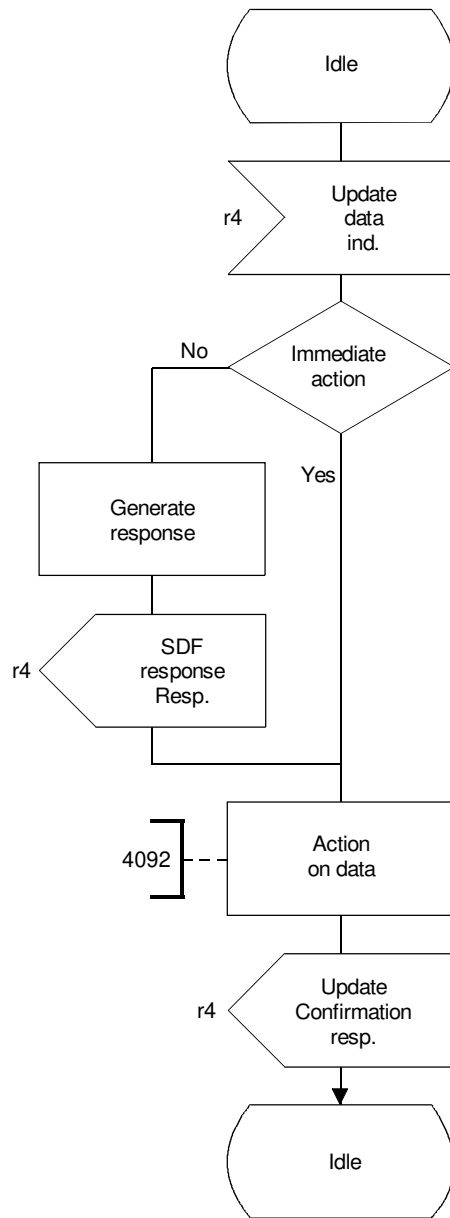
FIGURE 5-36/Q.1214 “Service data management” SIB service data functional entity
