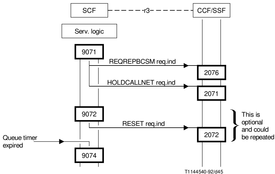
FIGURE 5-21/Q.1214 Information flow for queue SIB (queue without announcement)
