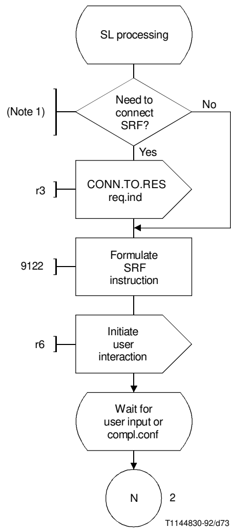
FIGURE 5-47/Q.1214 (sheet 1 of 2) User interaction SCF
