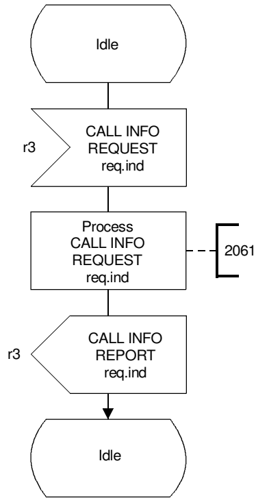
FIGURE 5-19/Q.1214 CCF/SSF actions for the “log call information” SIB
