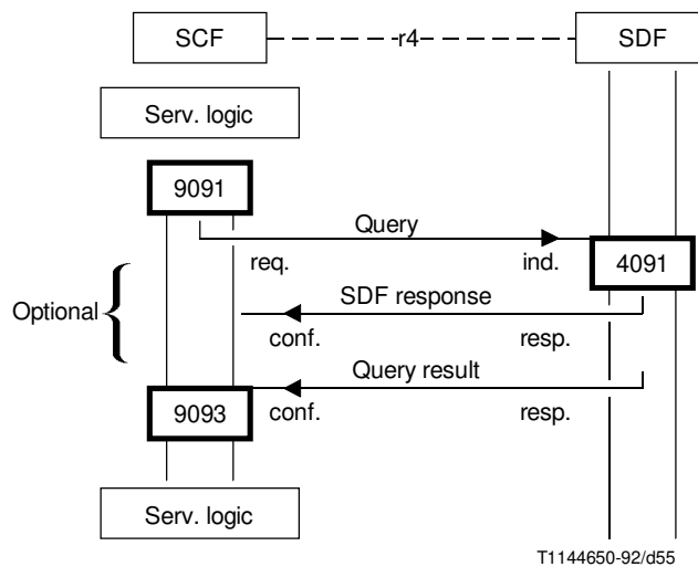
FIGURE 5-31/Q.1214 Information flow diagram “service data management” SIB (retrieve data)
