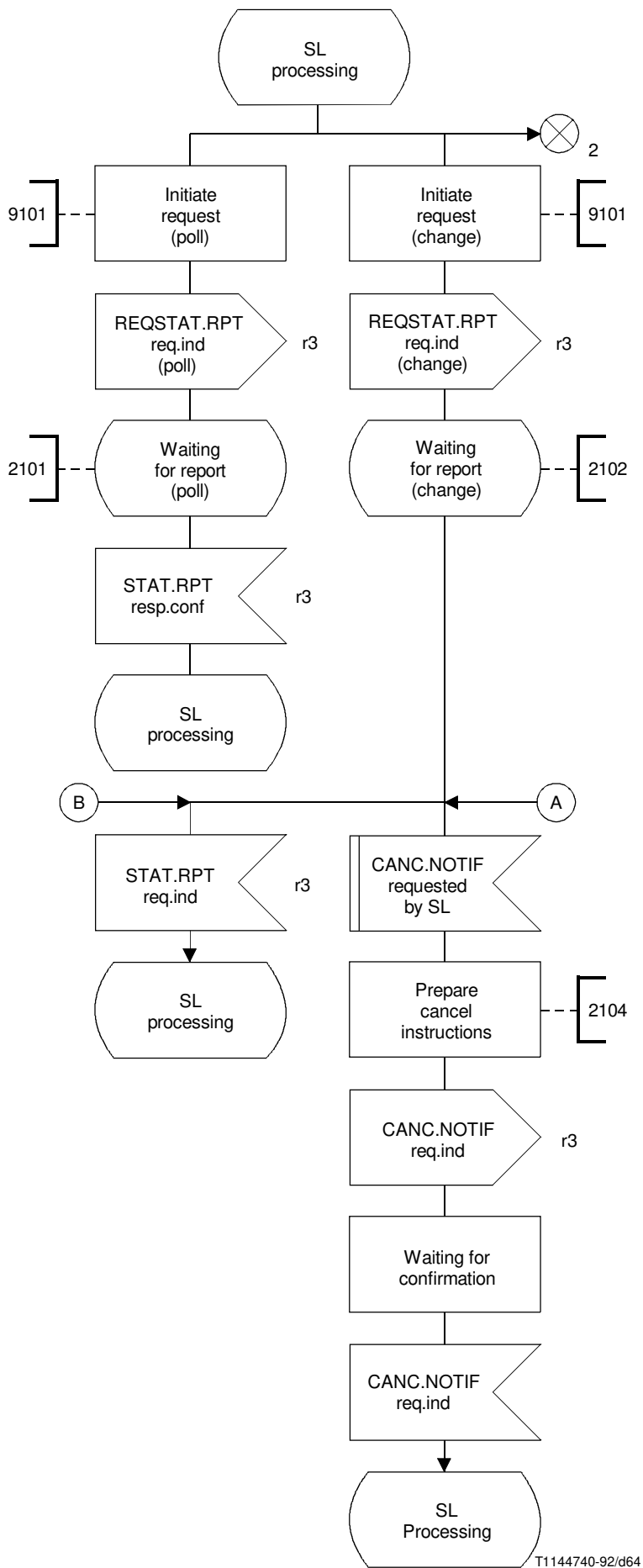
FIGURE 5-40/Q.1214 (sheet 1 of 2)
