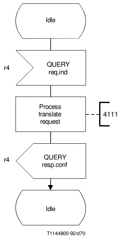
FIGURE 5-44/Q.1214 “Translate” SIB SDF entity
