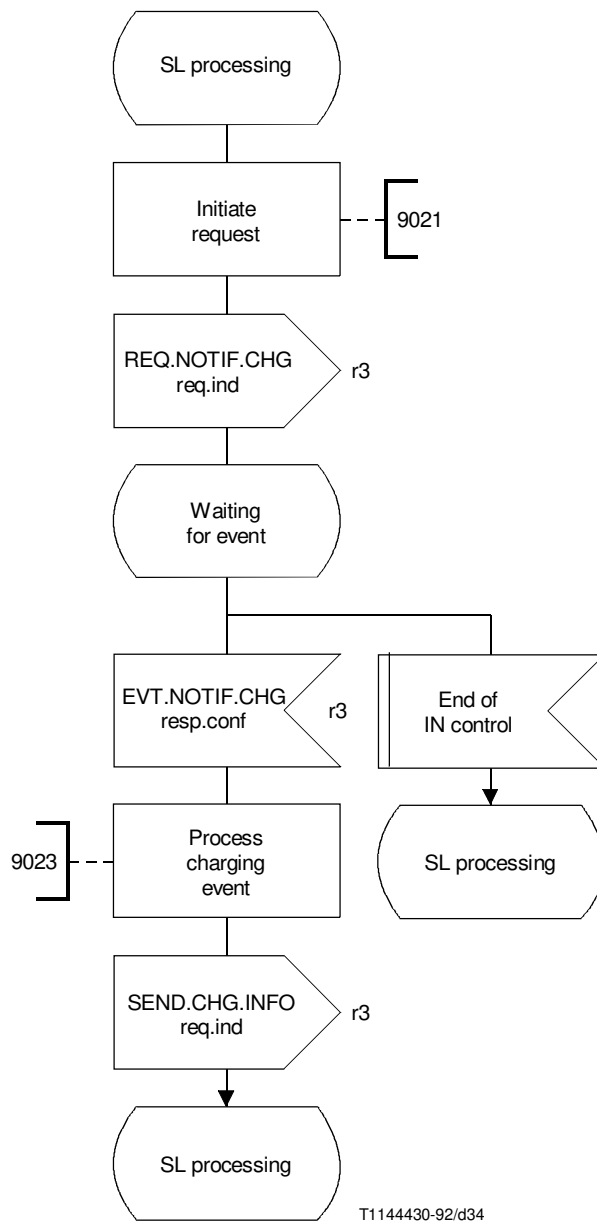
FIGURE 5-10/Q.1214 SCF-charging event “charge” SIB
