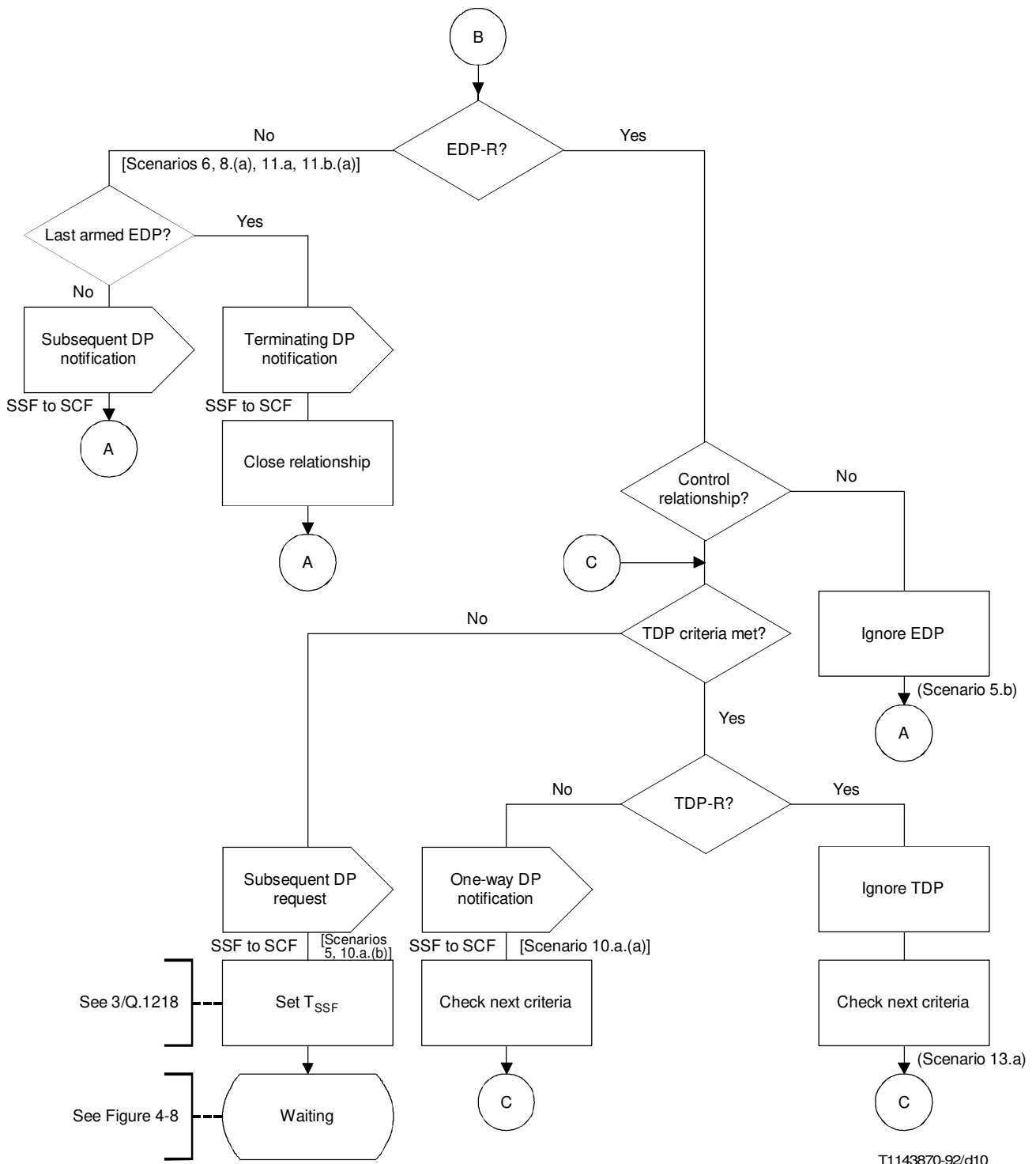
FIGURE 4-7/Q.1214 Detection point processing
