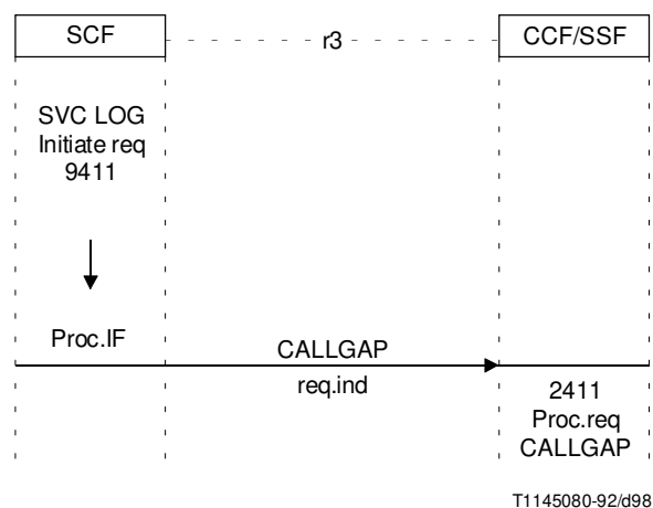
FIGURE 5-65/Q.1214 Information flow diagram call gap for service management
