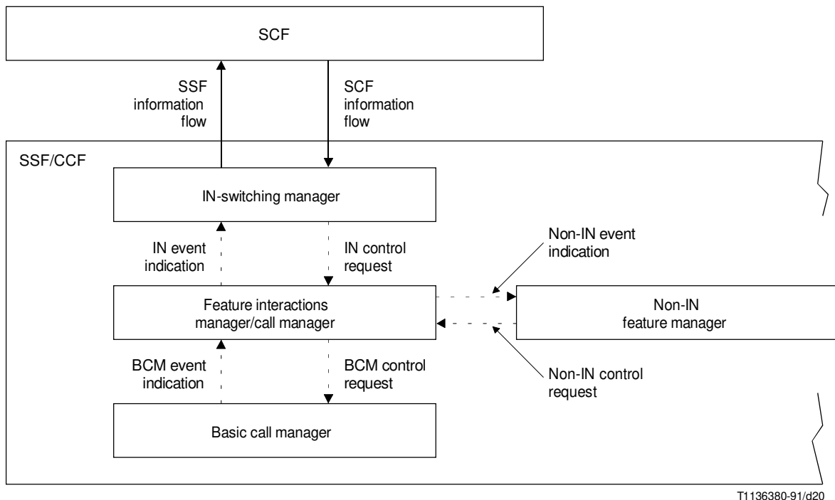
FIGURE 4-17/Q.1214 SSF/CCF model information flows
