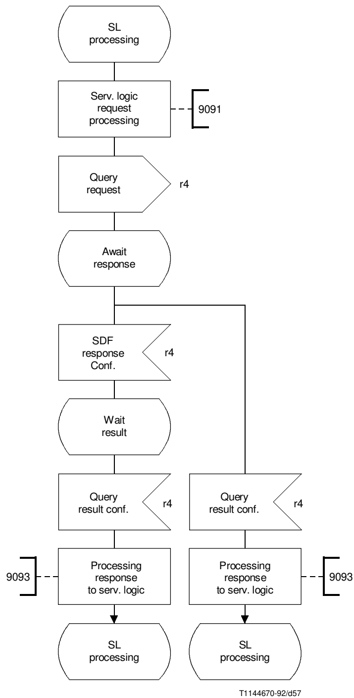
FIGURE 5-33/Q.1214 “Service data management” SIB service control functional entity
