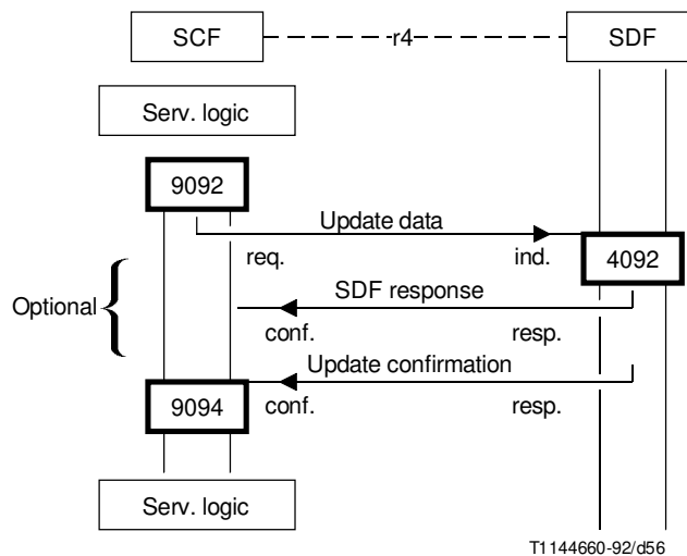
FIGURE 5-32/Q.1214 Information flow diagram “service data management” SIB (action on data)
