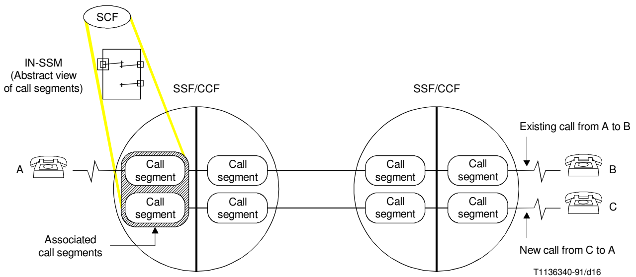
FIGURE 4-13/Q.1214 Associated call segments
