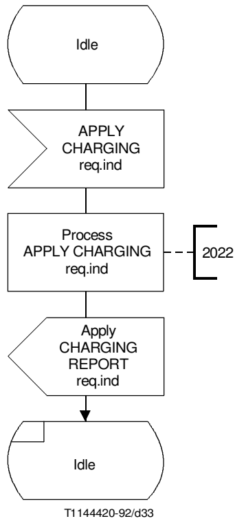
FIGURE 5-9/Q.1214 CCF/SSF actions for the “charge” SIB
