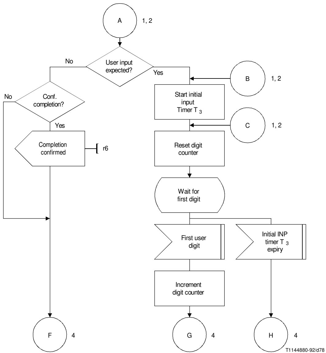
FIGURE 5-49/Q.1214 (sheet 3 de 5) User interaction SRF
