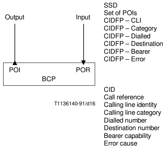
FIGURE 16/Q.1213 Basic call process SIB
