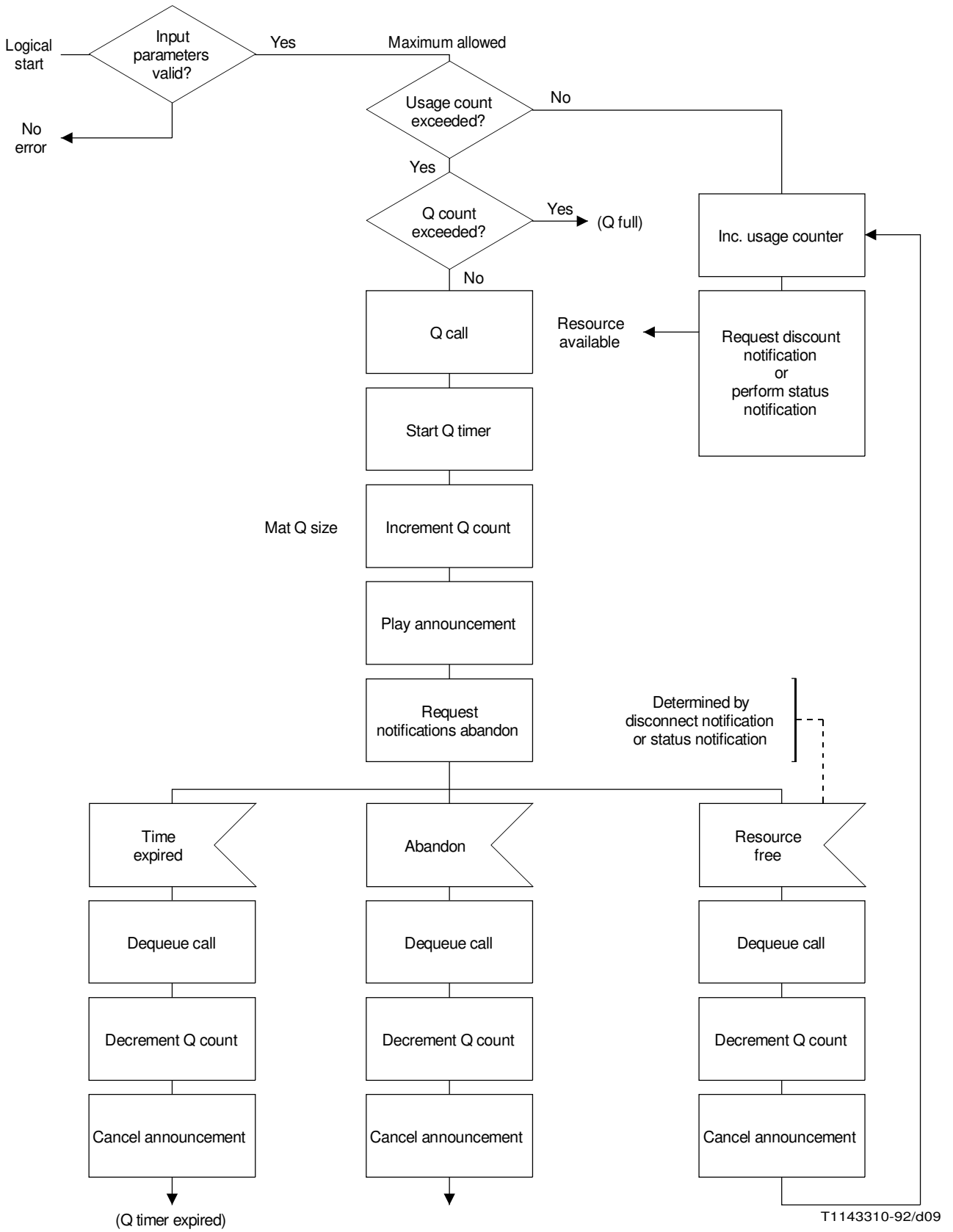
FIGURE 9/Q.1213 Queue SIB stage 1
