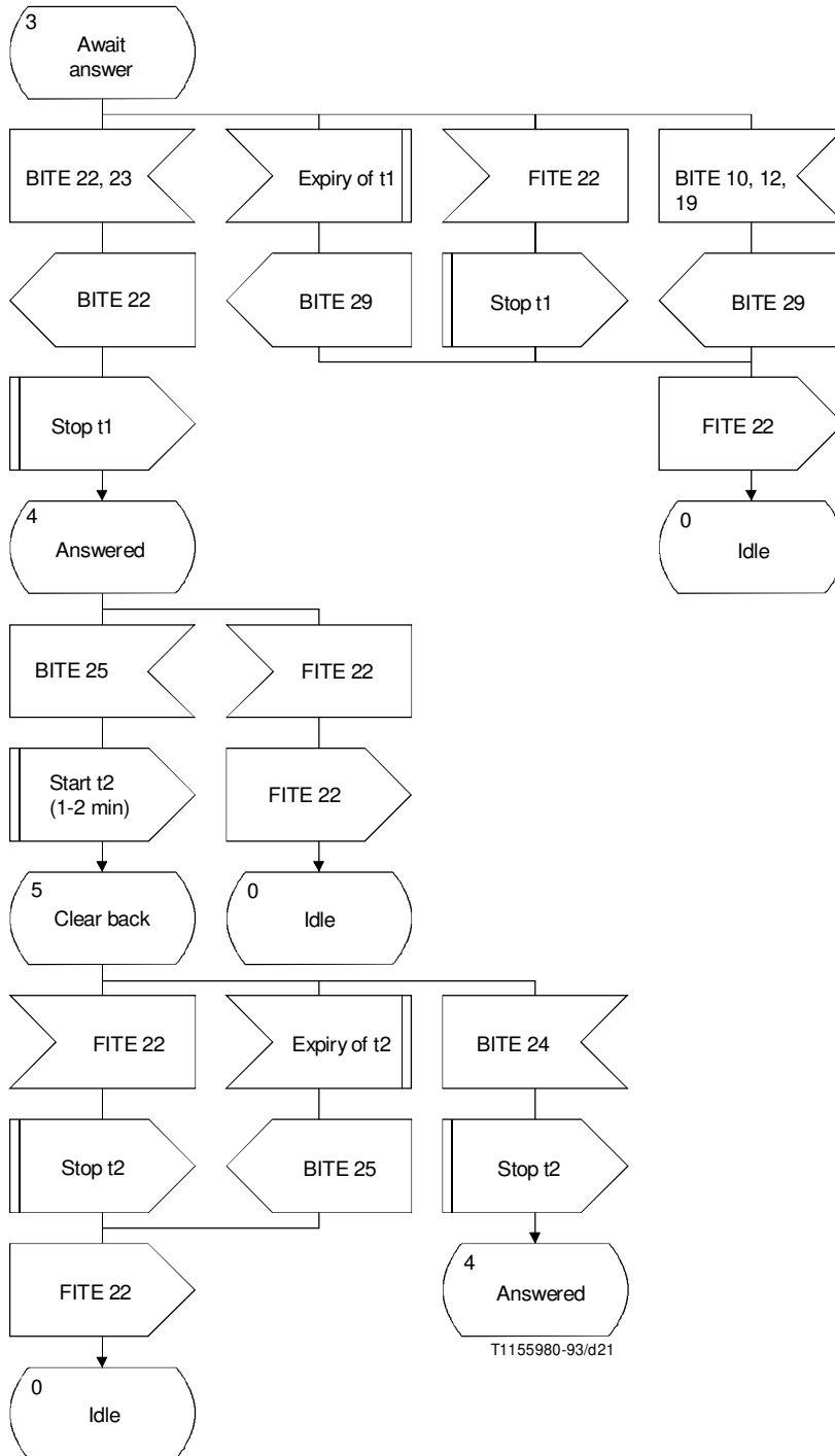
FIGURE 6/Q.1152 (sheet 3 of 3) Interworking of INMARSAT aeronautical system to Signalling System No. 7 TUP
