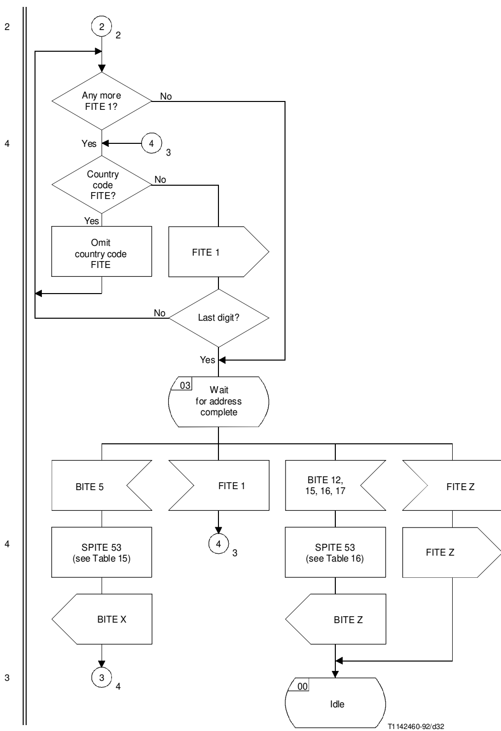
FIGURE 11/Q.1152 (sheet 3 of 4)
