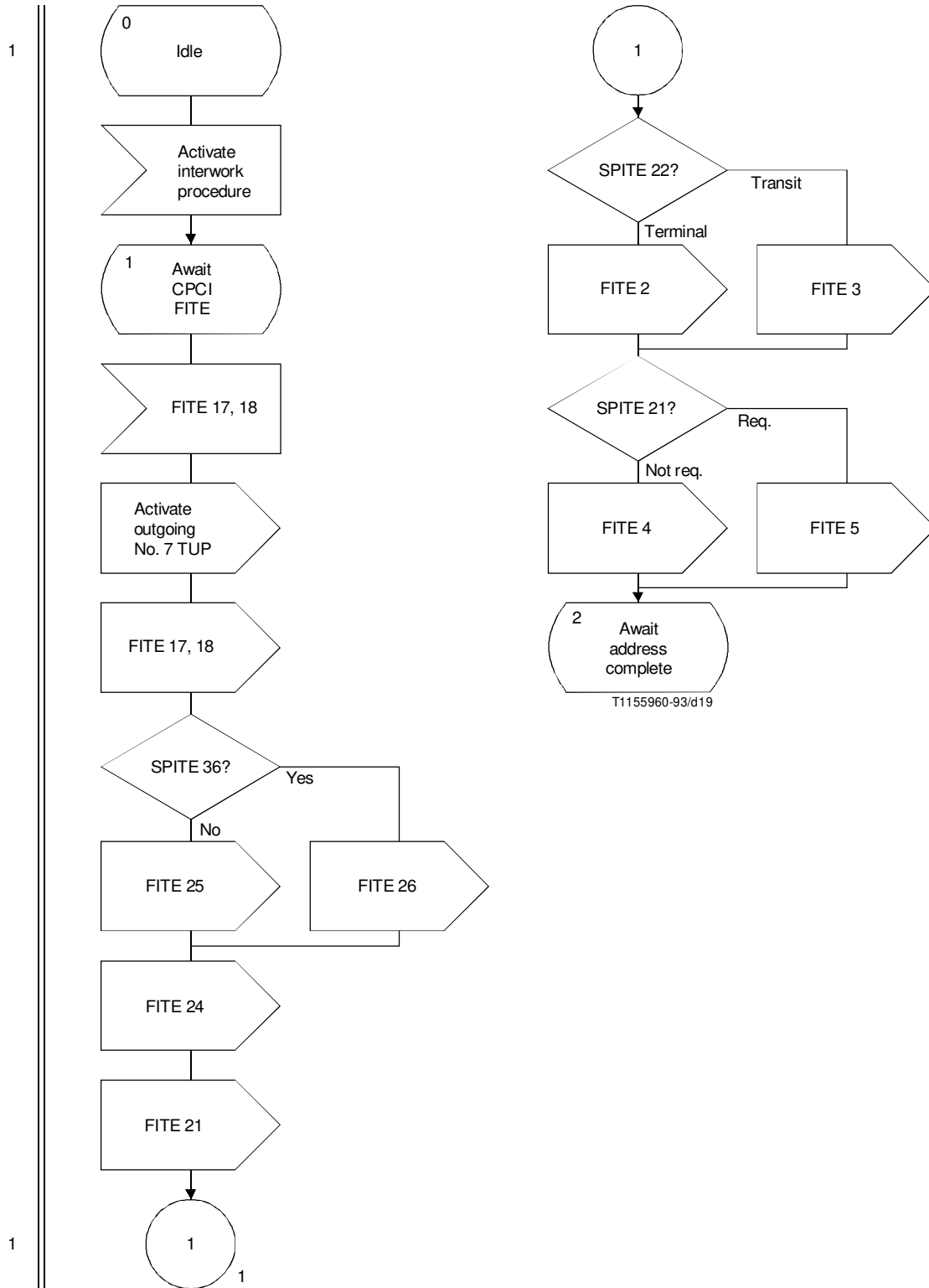
FIGURE 6/Q.1152 (sheet 1 of 3)
