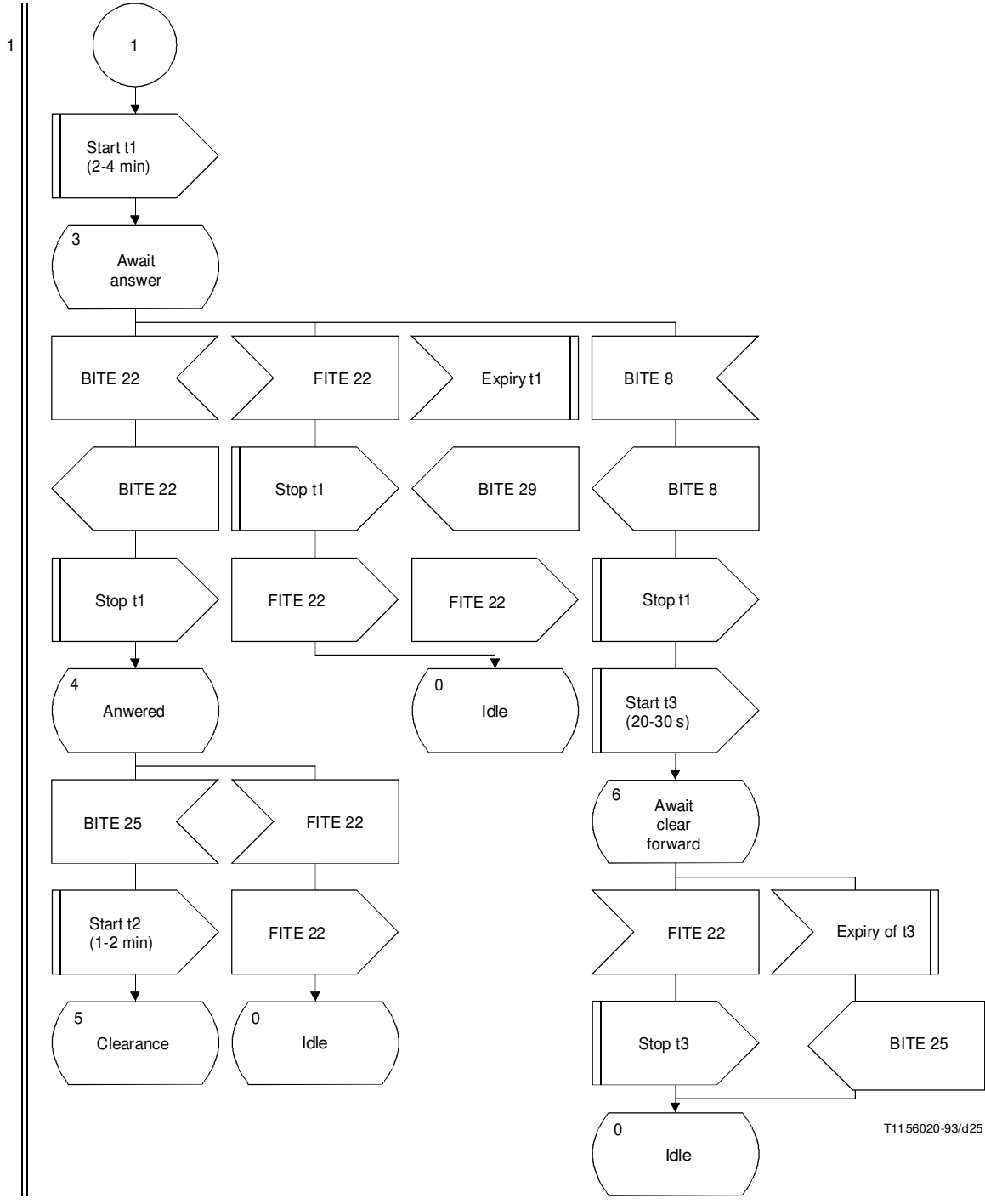
FIGURE 8/Q.1152 (sheet 2 of 3) Interworking of INMARSAT aeronautical system to Signalling System No. 5
