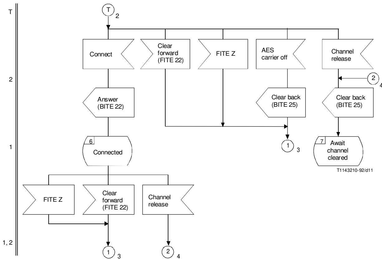
FIGURE 2/Q.1152 (sheet 4 of 4) Logic procedures for outgoing INMARSAT aeronautical signalling (ground-to-air-calls)
