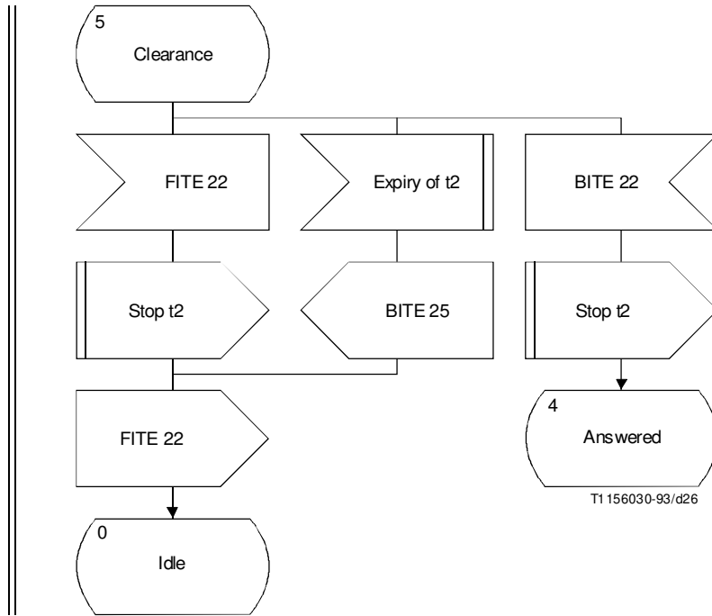
FIGURE 8/Q.1152 (sheet 3 of 3) Interworking of INMARSAT aeronautical system to Signalling System No. 5
