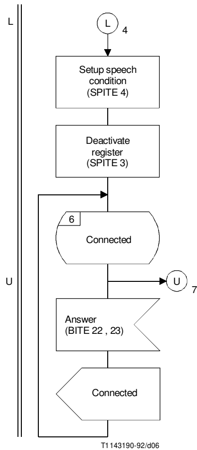
FIGURE 1/Q.1152 (sheet 6 of 7) Logic procedures for incoming INMARSAT aeronautical signalling (air-to-ground calls)
