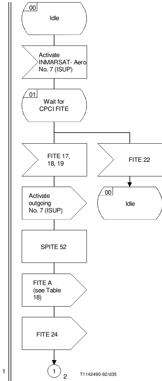
FIGURE 13/Q.1152 (sheet 1 of 5)
