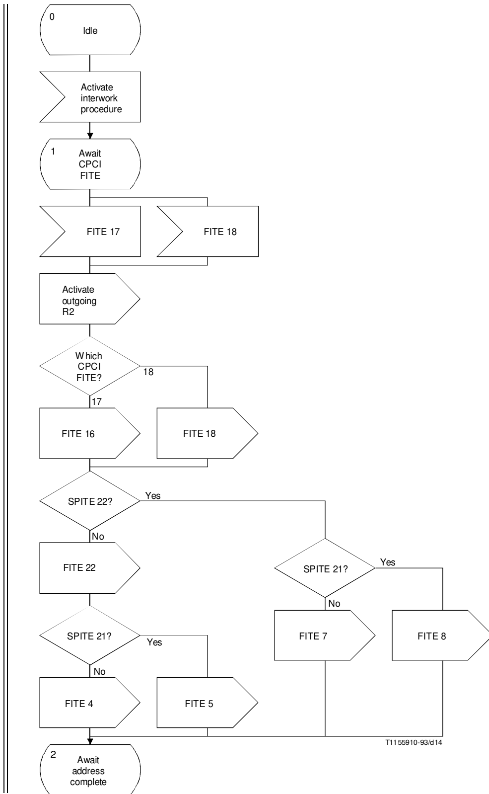
FIGURE 4/Q.1152 (sheet 1 of 3) Interworking of INMARSAT aeronautical system to Signalling System R2
