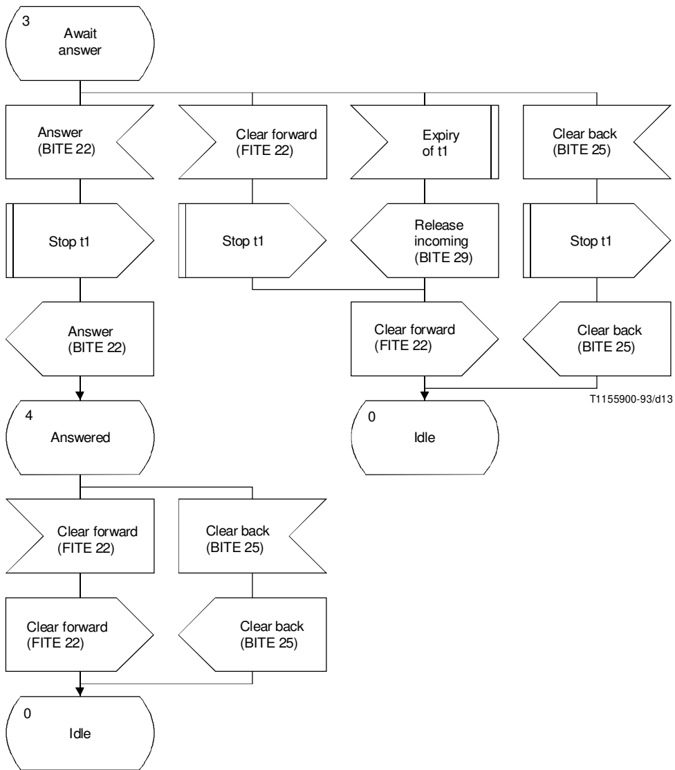
FIGURE 3/Q.1152 (sheet 2 of 2) Interworking of INMARSAT aeronautical system with itself
