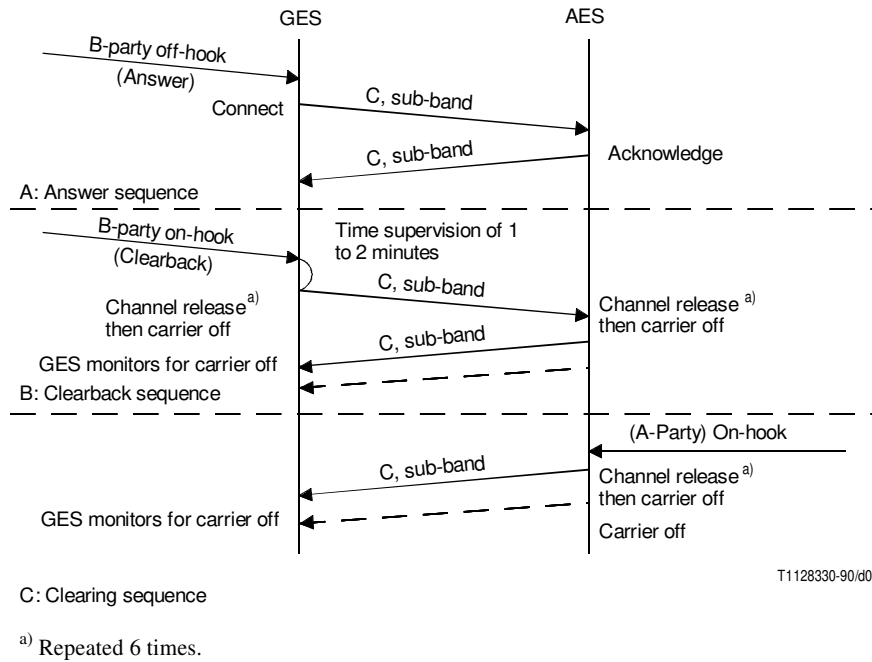
FIGURE I.6/Q.1151 Air-to-ground telephone call user switchhook signalling
