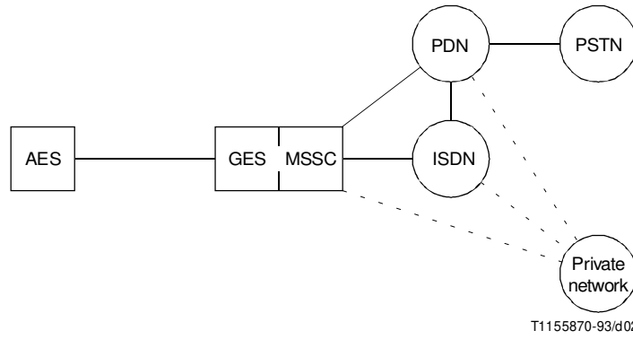
FIGURE 2/Q.1151 Interim interworking scenario with interfaces to ISDN and other fixed networks
