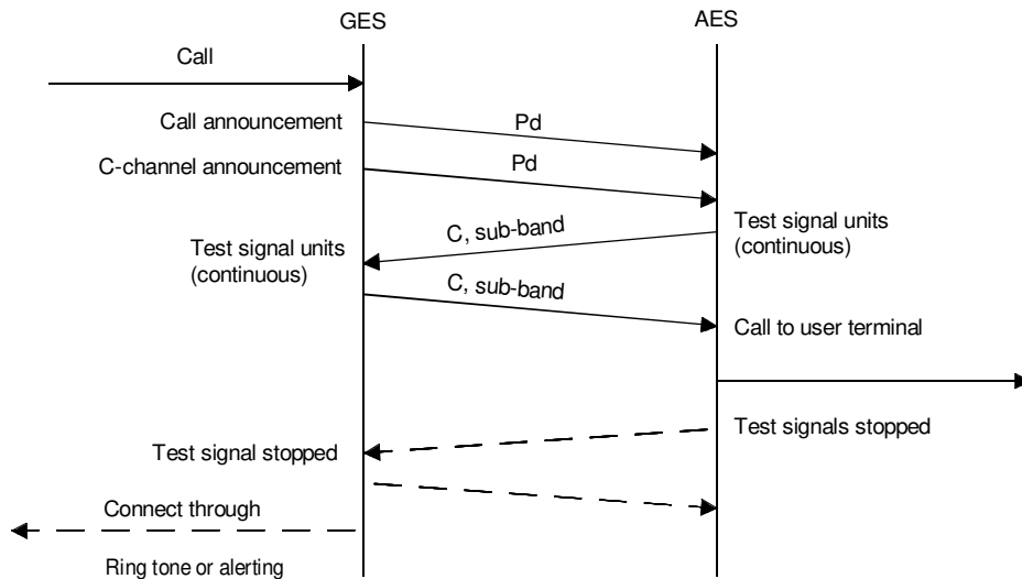
FIGURE I.7/Q.1151 Ground-to-air telephone call set-up sequence
