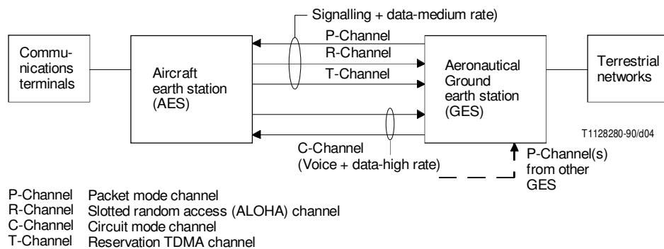
FIGURE I.1/Q.1151 Aeronautical network configuration
