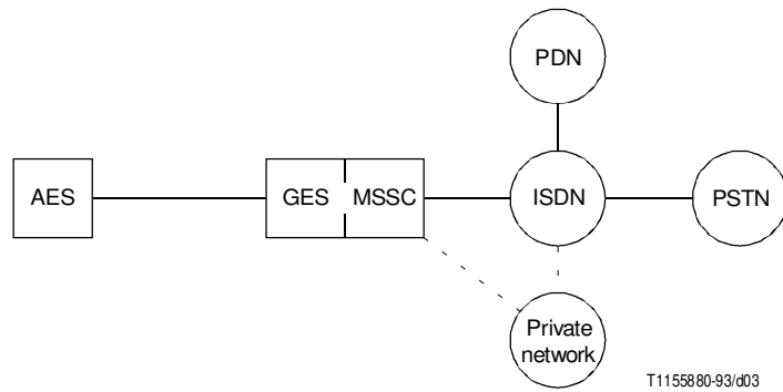
FIGURE 3/Q.1151 Interworking scenario with ISDN interface only
