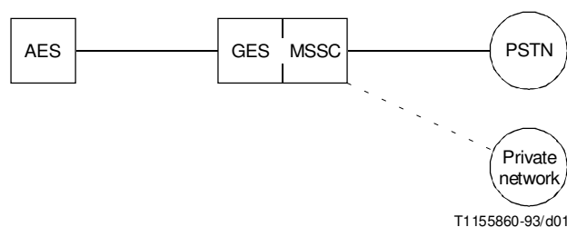
FIGURE 1/Q.1151 Interworking scenario with PSTN interface
