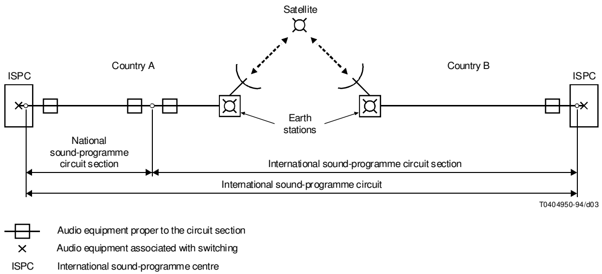
FIGURE 3/N.1 Single-destination international sound-programme circuit routed via a communication satellite system
