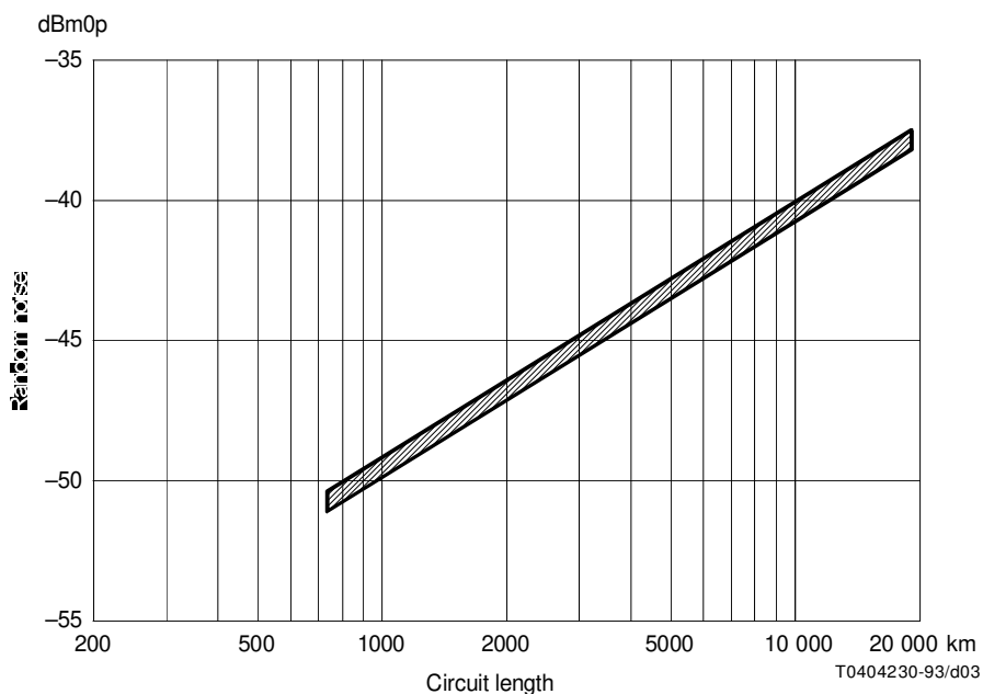
FIGURE 3/M.4030 Random noise performance
