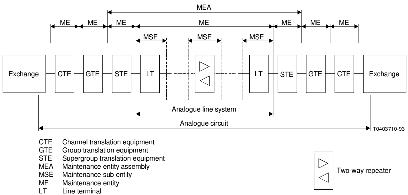
FIGURE 3/M.20 Maintenance entity concept for analogue networks
