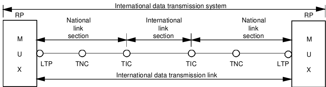
c) Multiplex/Demultiplex equipment located at the RP
