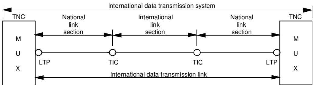
b) Multiplex/Demultiplex equipment located at the TNC
