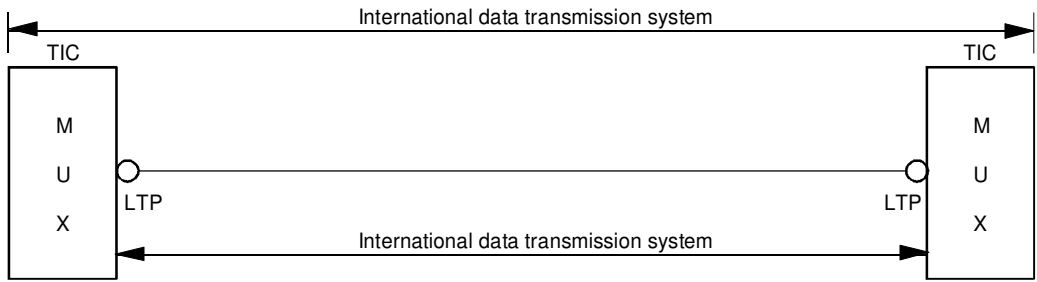
a) Multiplex/Demultiplex equipment located at the TIC
