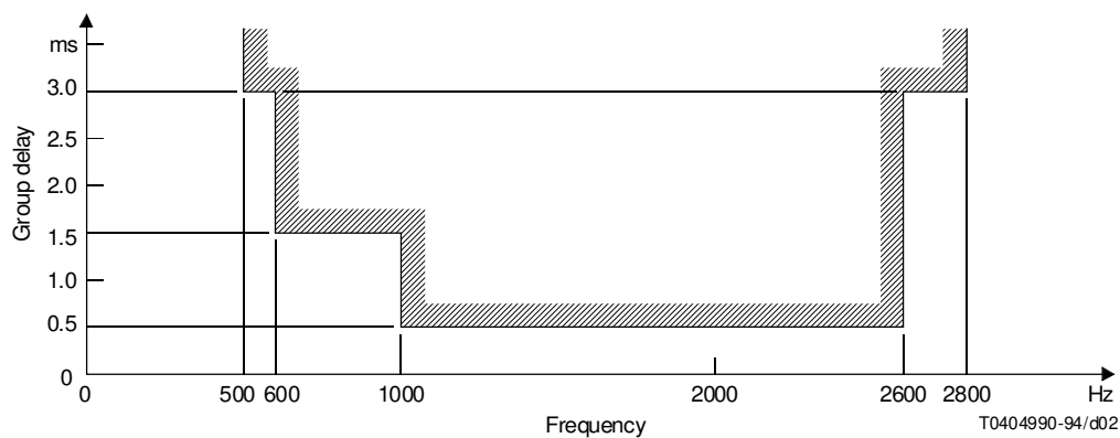
FIGURE 2/M.1020 Limits for group delay relative to the minimum measured group delay in the 500-2800 Hz band
