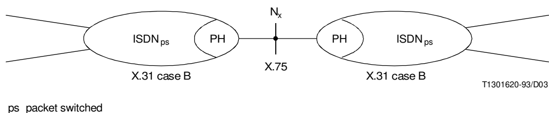
FIGURE 3/I.520 ISDN ps interworking with ISDN ps
