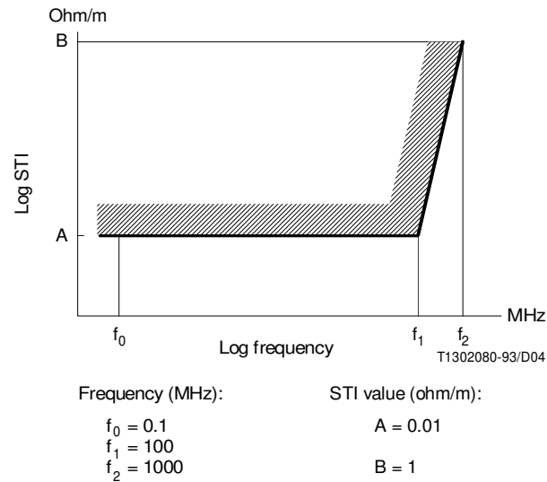
FIGURE 4/I.432 Maximum STI values as function of frequency
