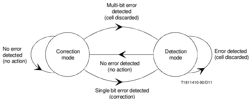
FIGURE 11/I.432 HEC: Receiver modes of operation
