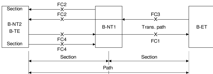
FIGURE 15/I.432 Fault conditions and operational span of section path maintenance signals
