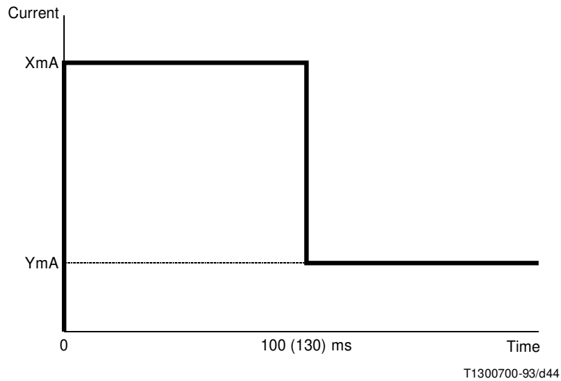
FIGURE I.6/I.430 Load L2 current VS time
