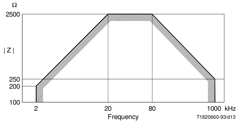
FIGURE 12/I.430 TE impedance template (log-log scale)
