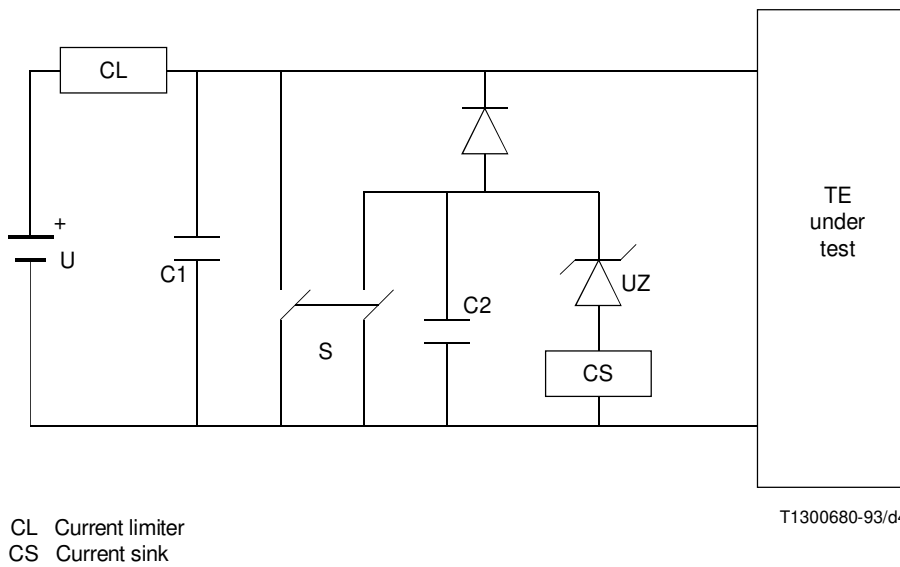
FIGURE I.3/I.430 Test circuit for TE start-up
