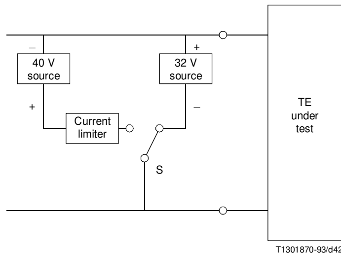
FIGURE I.4/I.430 TEST circuit for TE switchover
