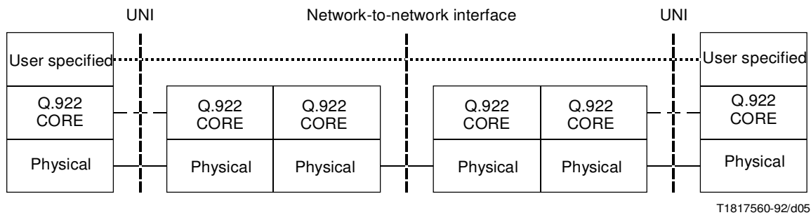
FIGURE 5/I.372 U-plane protocol reference architecture
