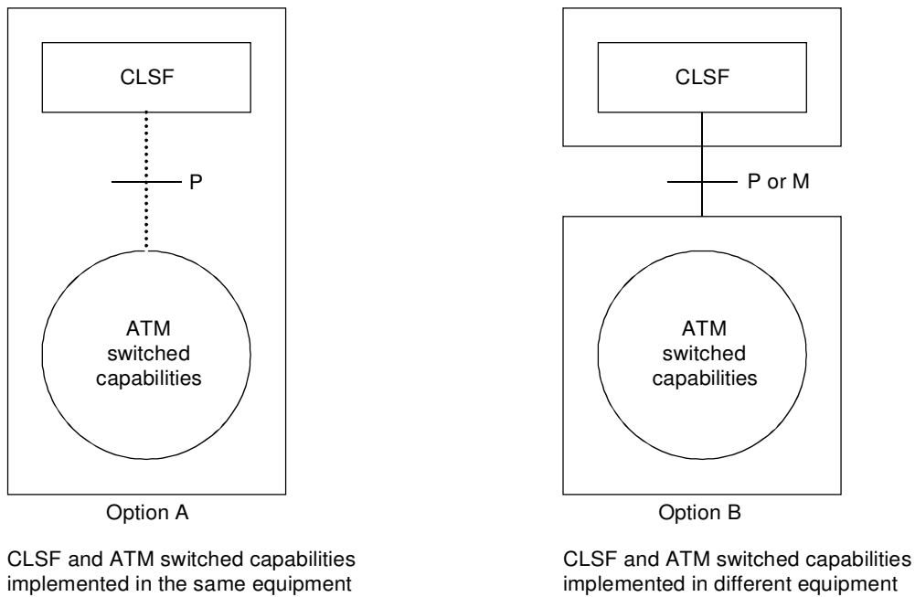
FIGURE 2/I.342 Implementation of CLSF and ATM switched capabilities
