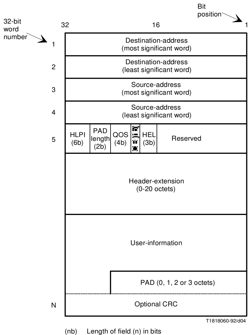
FIGURE 5/I.364 Structure of the CLNAP-PDU
