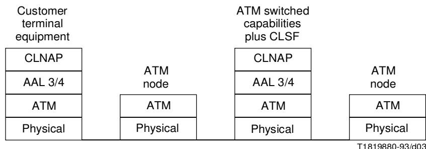
FIGURE 3/I.364 General protocol structure for provision of CL data service in B-ISDN
