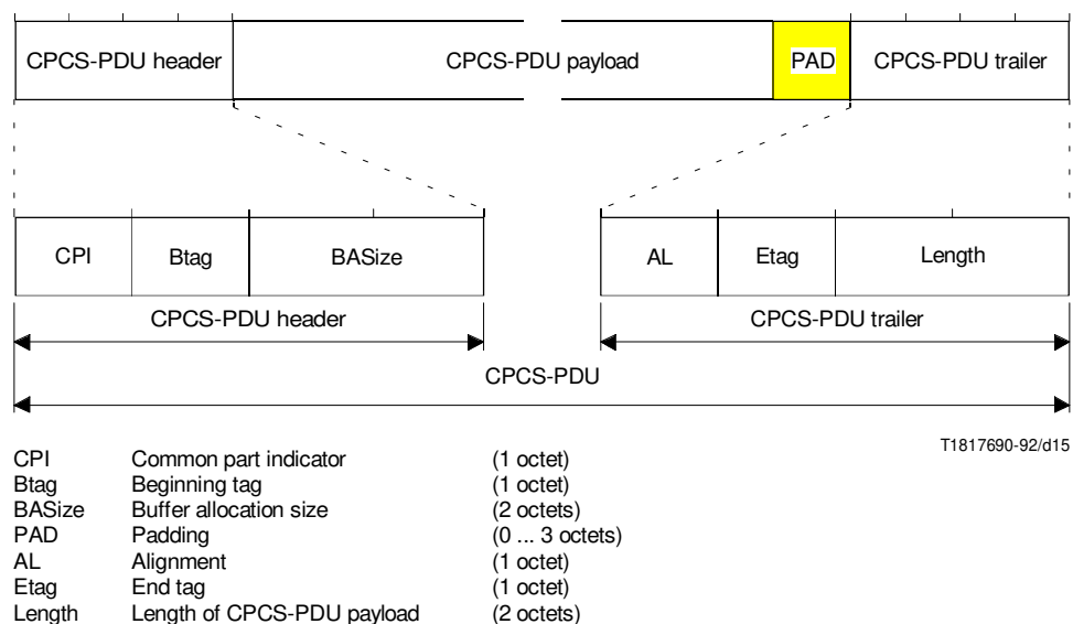
FIGURE 15/I.363 CPCS-PDU format for AAL type 3/4
