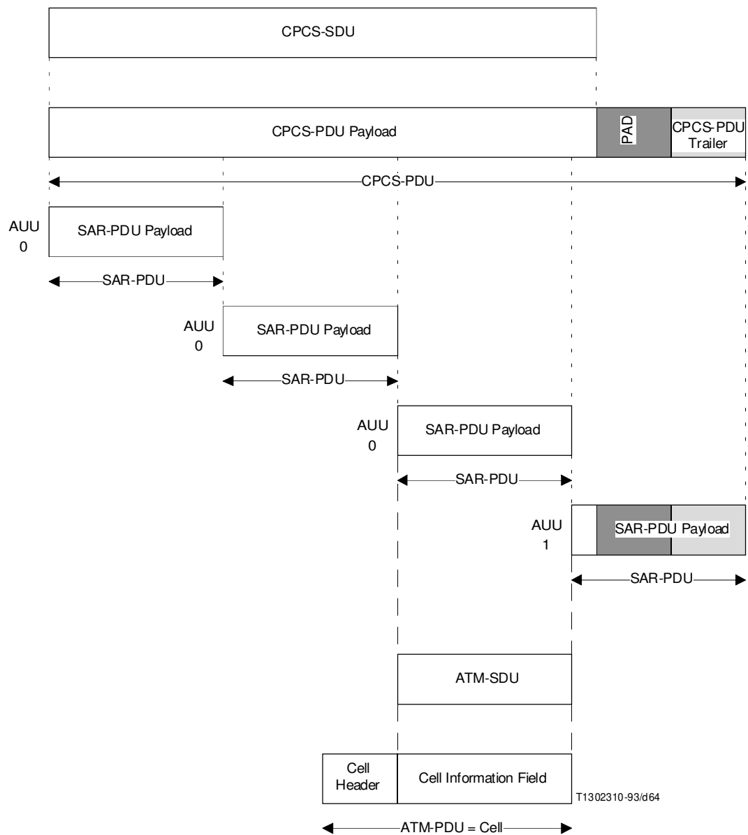
FIGURE F.2/I.363 PDU Headers, trailers and terminology
