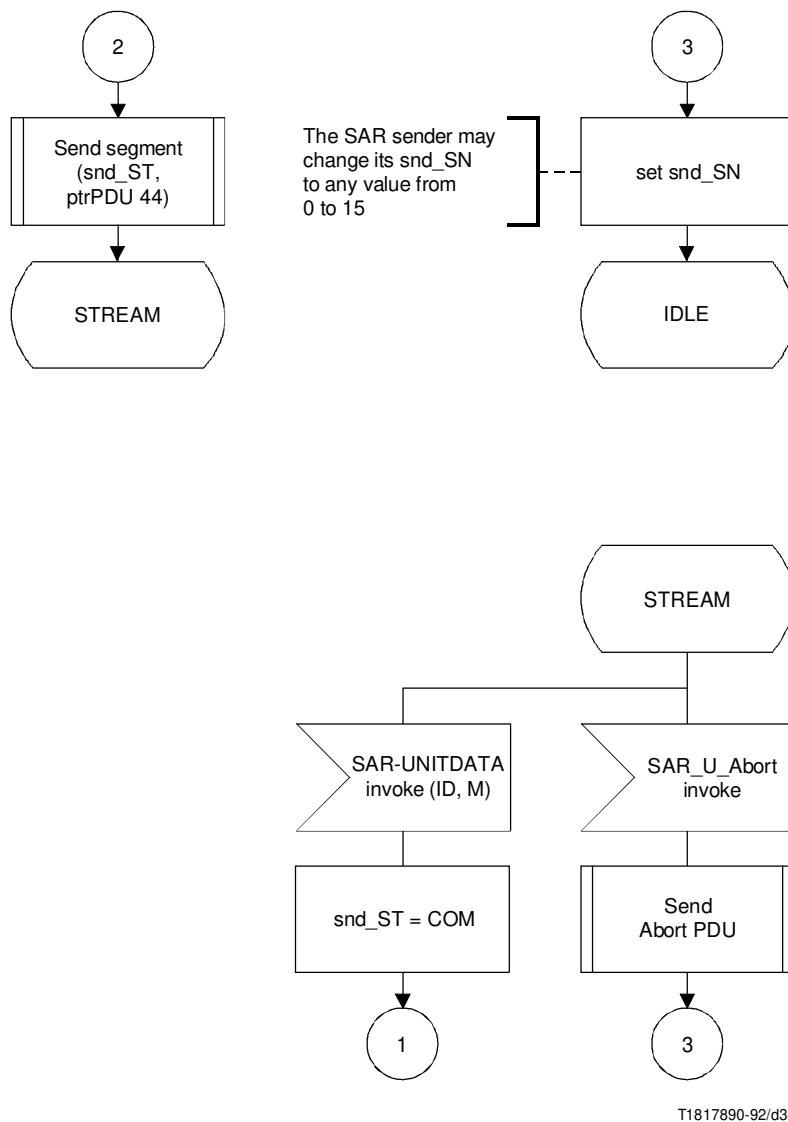
FIGURE I.1/I.363 (sheet 3 of 5)
