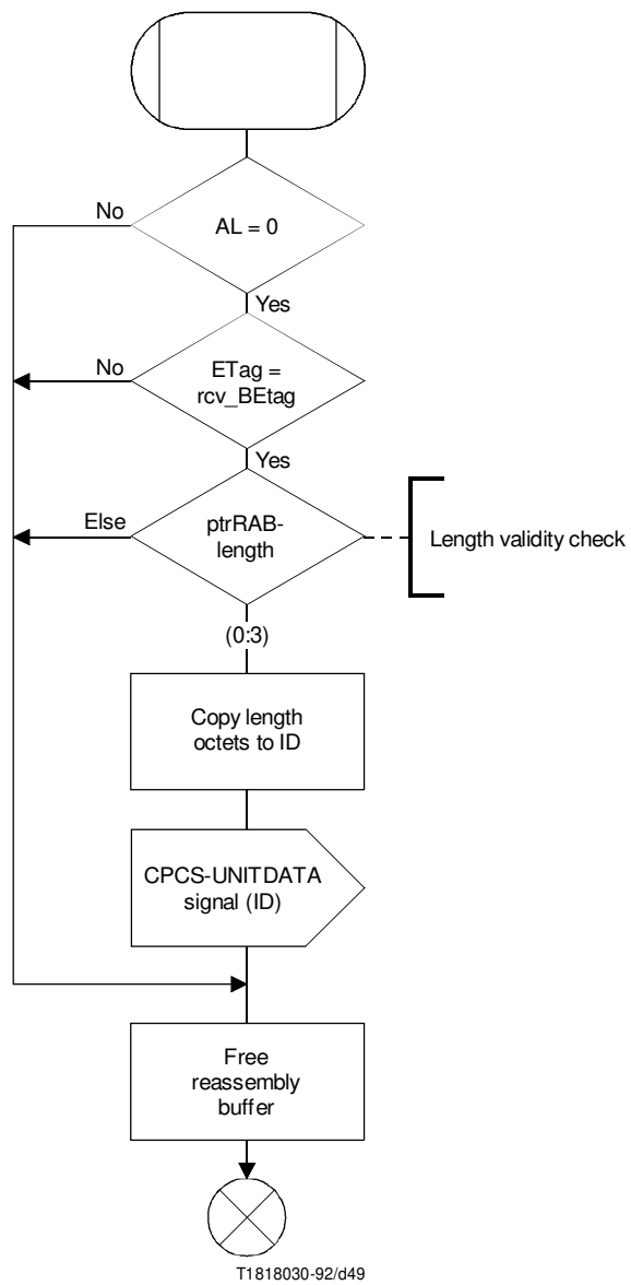
FIGURE I.5/I.363 (sheet 5 of 5)
