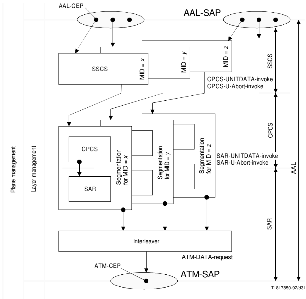
FIGURE C.1/I.363 Functional model for the AAL Type 3/4 (Sender side)
