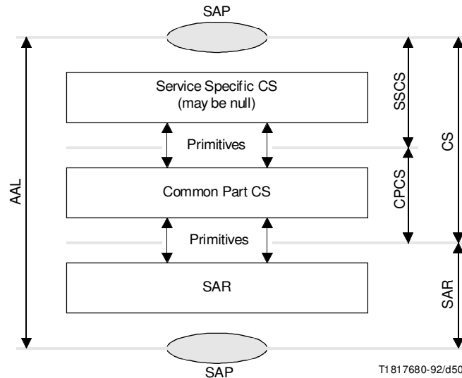
FIGURE 6-1/I.363 Structure of the AAL type 5
