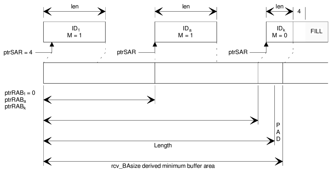
FIGURE I.3/I.363 The mechanism of the reassembly buffer
