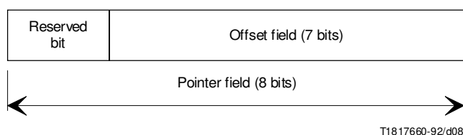
FIGURE 8/I.363 Pointer field format
