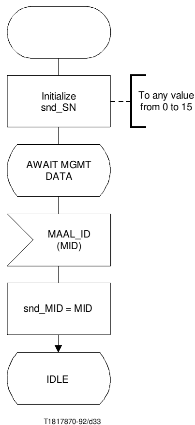
FIGURE I.1/I.363 (sheet 1 of 5)
