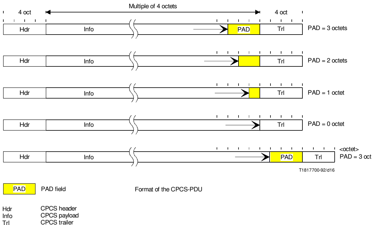
FIGURE 16/I.363 Function of the PAD field
