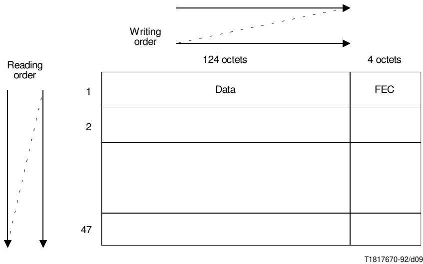
FIGURE 9/I.363 Format of the interleave matrix
