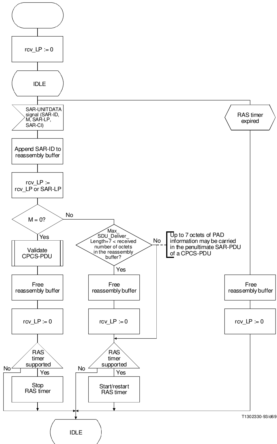
FIGURE II.4/I.363 SDL diagrams for the CPCS receiver
