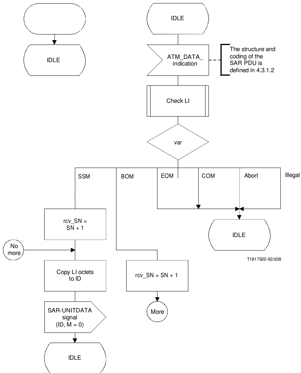
FIGURE I.2/I.363 (sheet 1 of 4)
