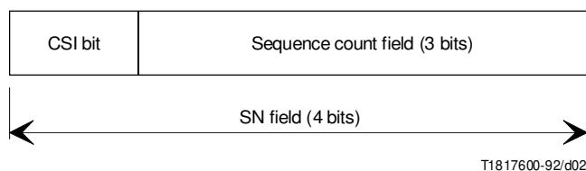
FIGURE 2/I.363 Sequence number (SN) field format
