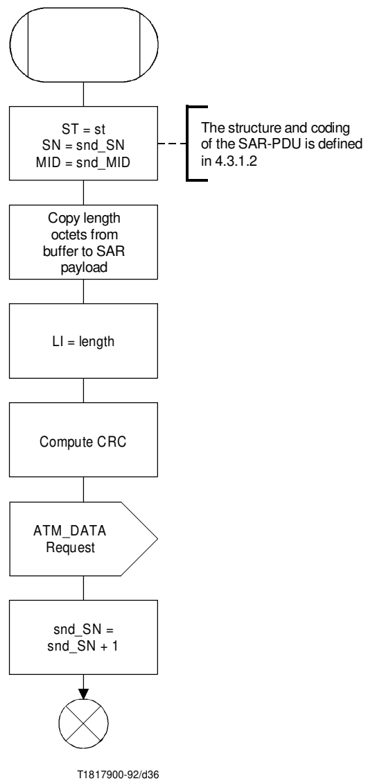
FIGURE I.1/I.363 (sheet 4 of 5)
