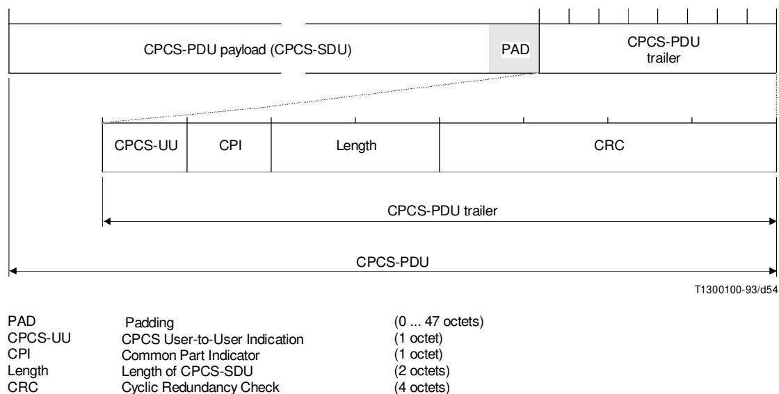
FIGURE 6-5/I.363 CPCS-PDU Format for the AAL type 5
