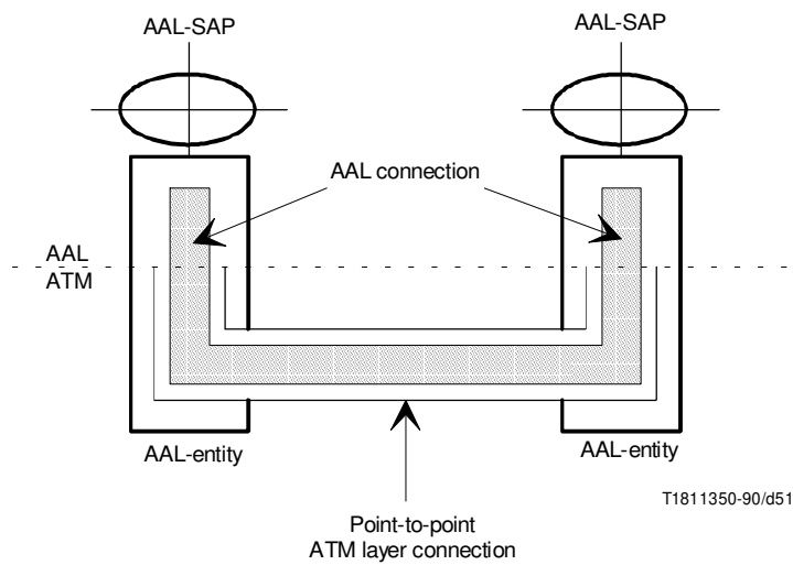
a) Point-to-point AAL connection
