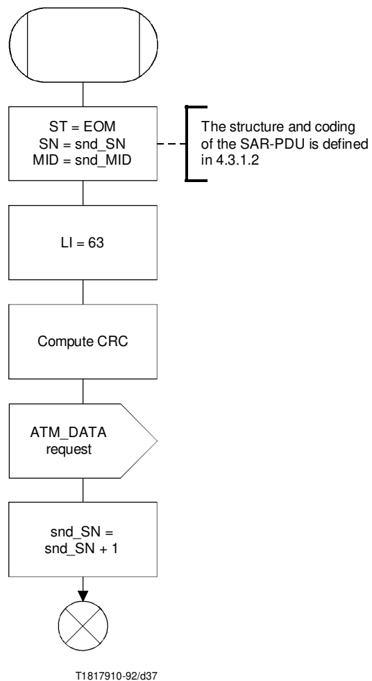
FIGURE I.1/L.363 (sheet 5 of 5)
