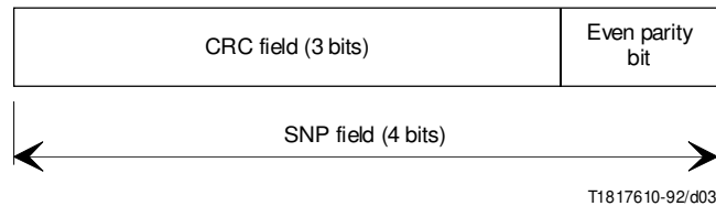
FIGURE 3/I.363 SNP field format
