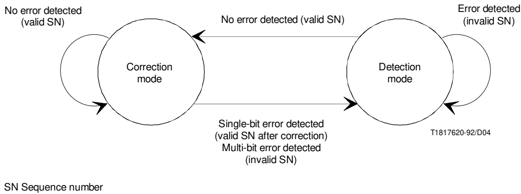
FIGURE 4/L363 SNP: receiver modes of operation
