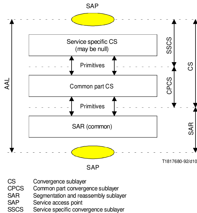
FIGURE 10/L.363 Structure of the AAL type 3/4
