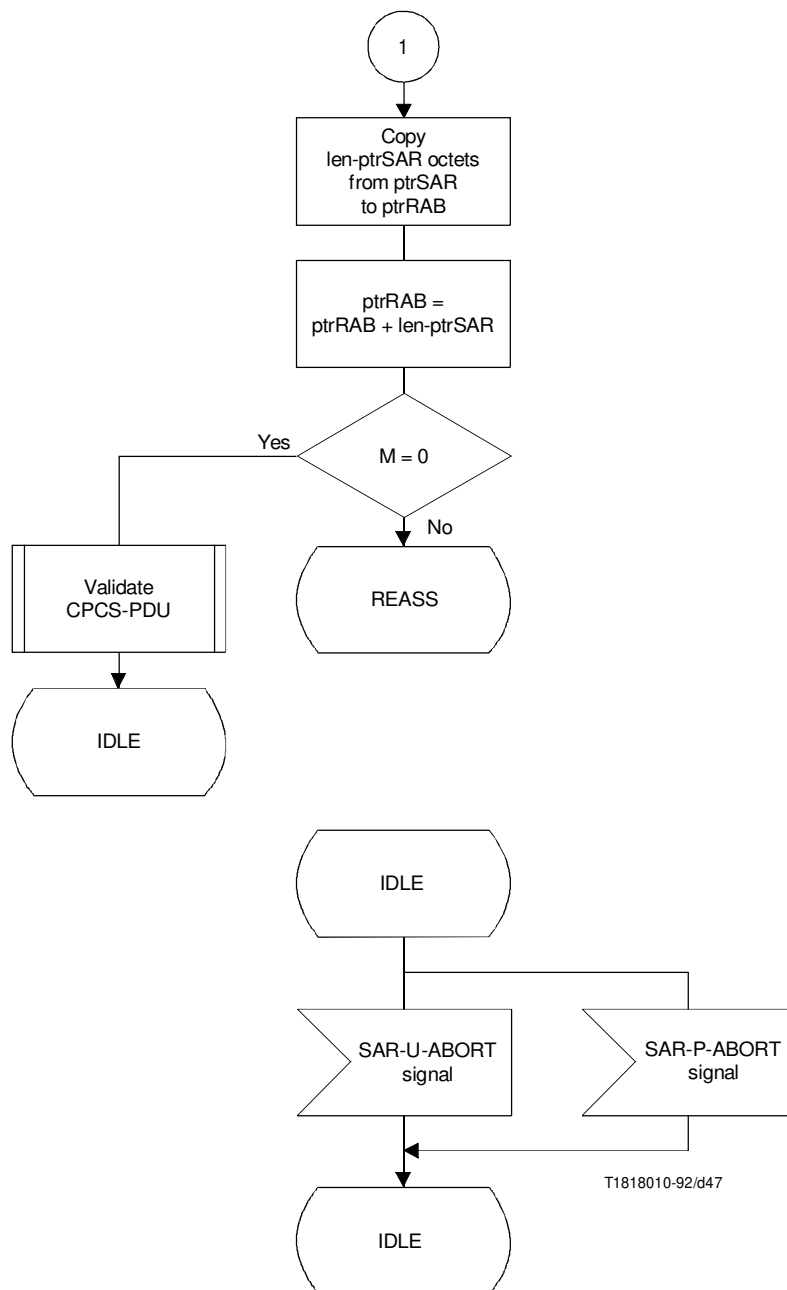
FIGURE I.5/I.363 (sheet 3 of 5)
