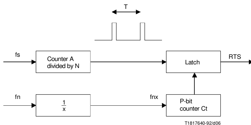
FIGURE 6/I.363 Generation of residual time stamp (RTS)
