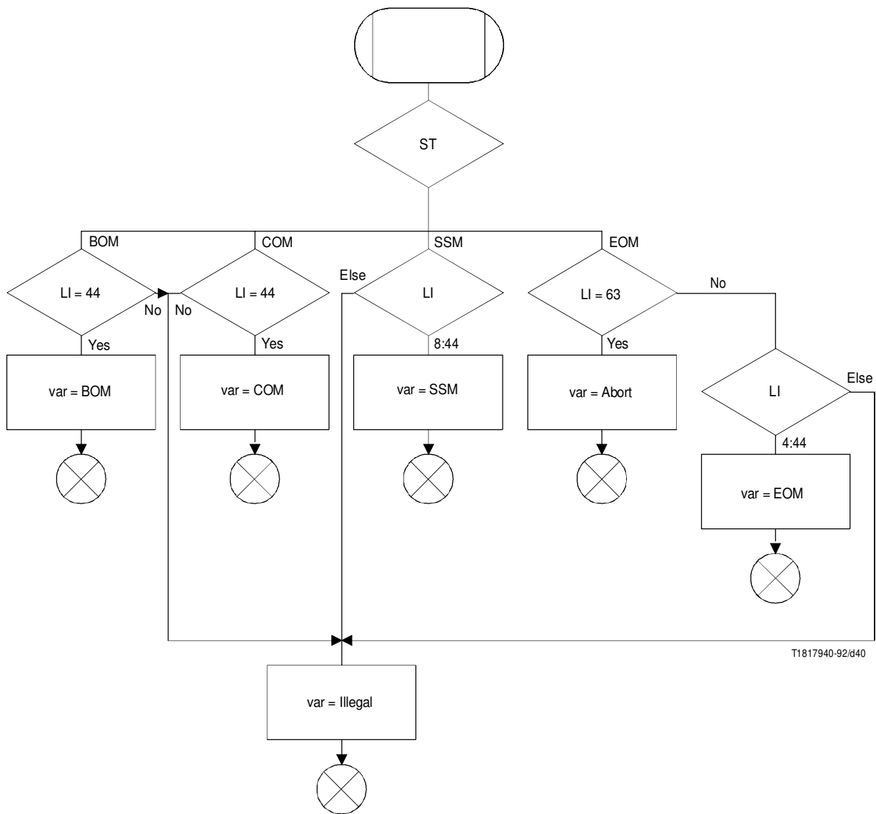
FIGURE I.2/I.363 (sheet 3 of 4)
