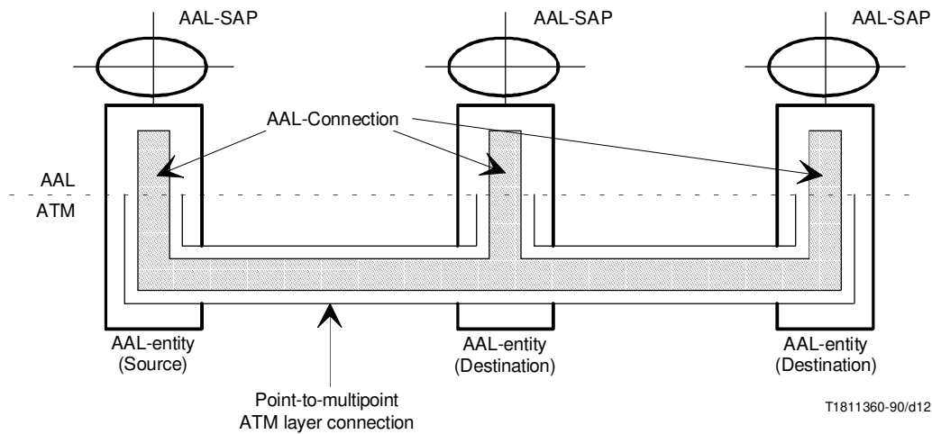
FIGURE 12/I.363 Point-to-multipoint AAL connection
