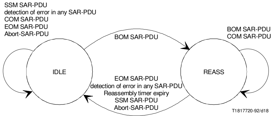
FIGURE 18/I.363 State transition diagram for the SAR receiver
