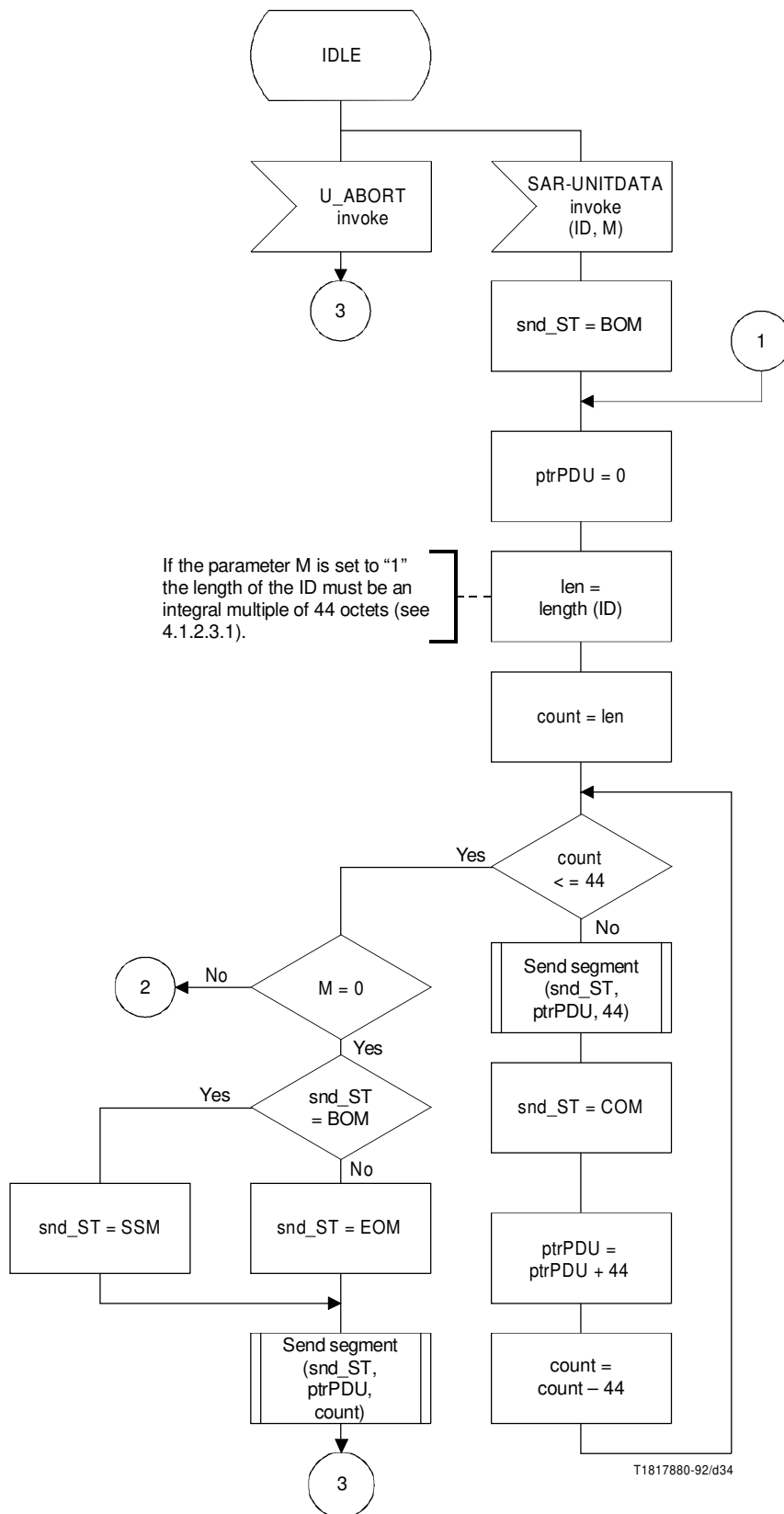
FIGURE I.1/I.363 (sheet 2 of 5)
