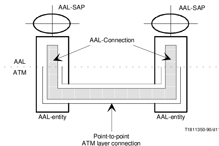
FIGURE 11/I.363 Point-to-point AAL connection
