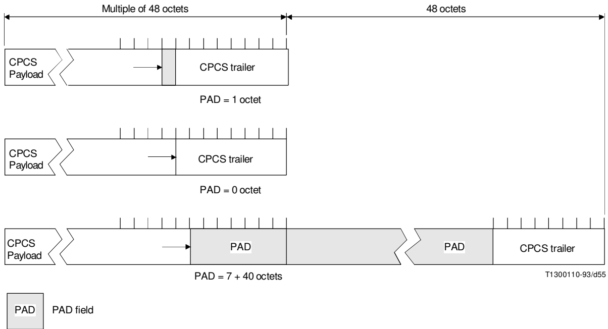
FIGURE 6-6/I.363 Examples of the PAD field function
