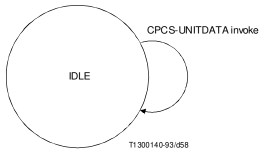
FIGURE 6-9/I.363 State transition diagram for the CPCS sender
