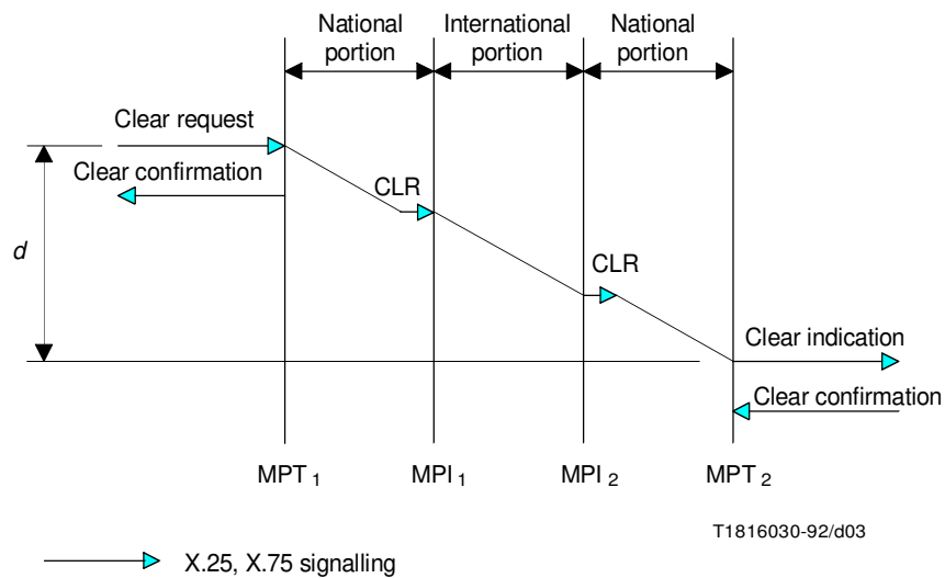
FIGURE A.3/I.354 End-to-end clear indication delay
