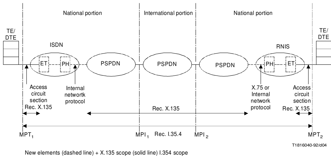
FIGURE I.1/I.354 Performance model comparison of X.135 and I.354 3)
