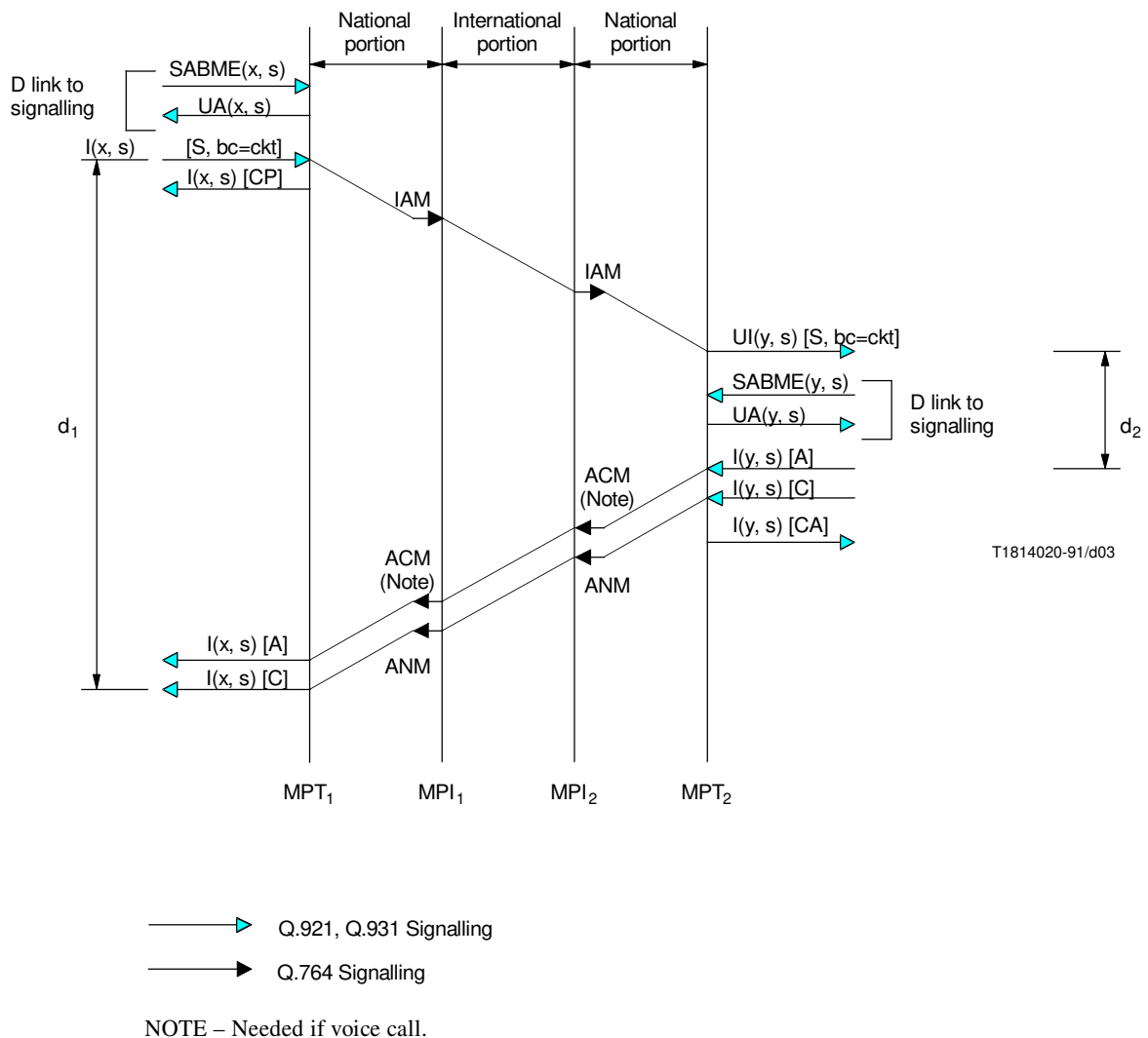
FIGURE 3/I.352 Alerting set-up delay
