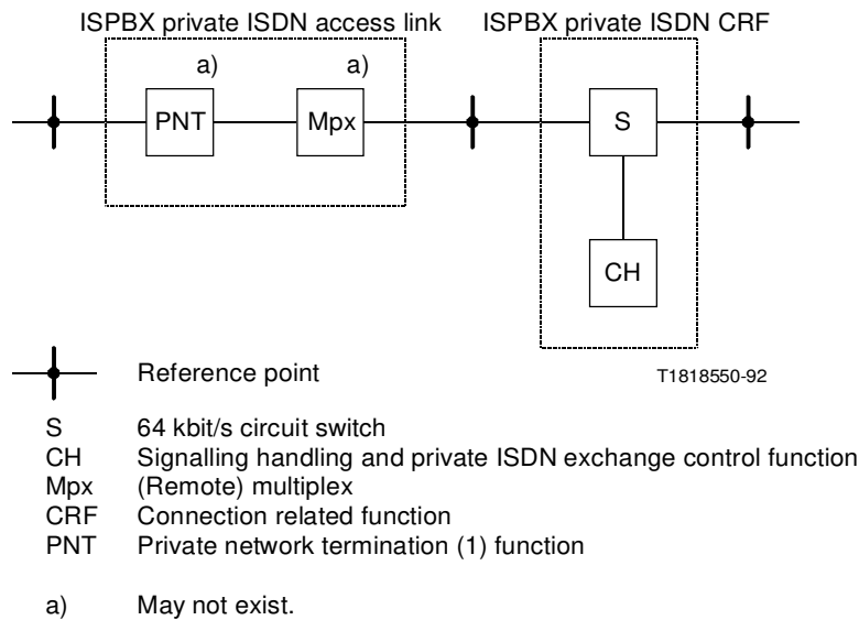
FIGURE 8/I.324 Private ISDN access connection element
