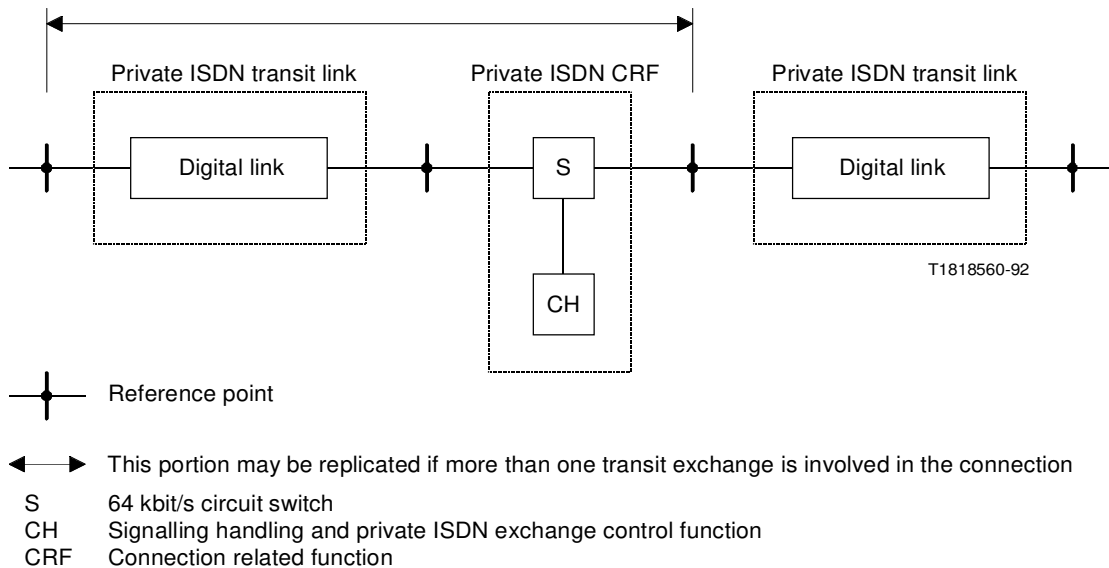
FIGURE 9/I.324 Private ISDN transit connection element
