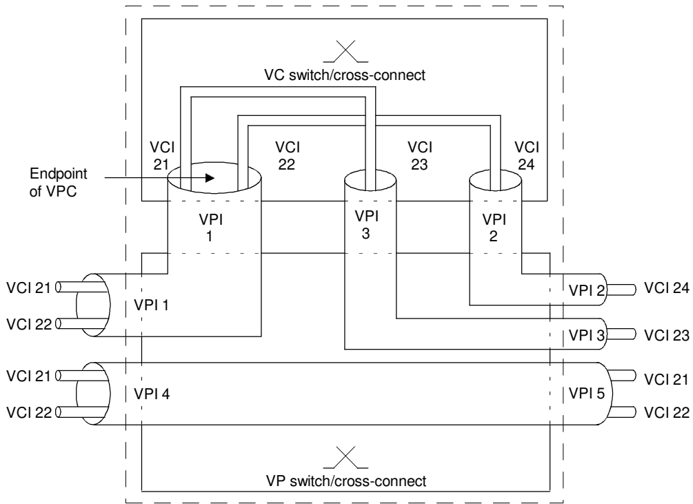
a) Representation of VC and VP switching
