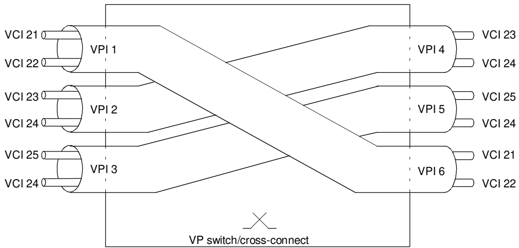
b) Representation of VP switching
