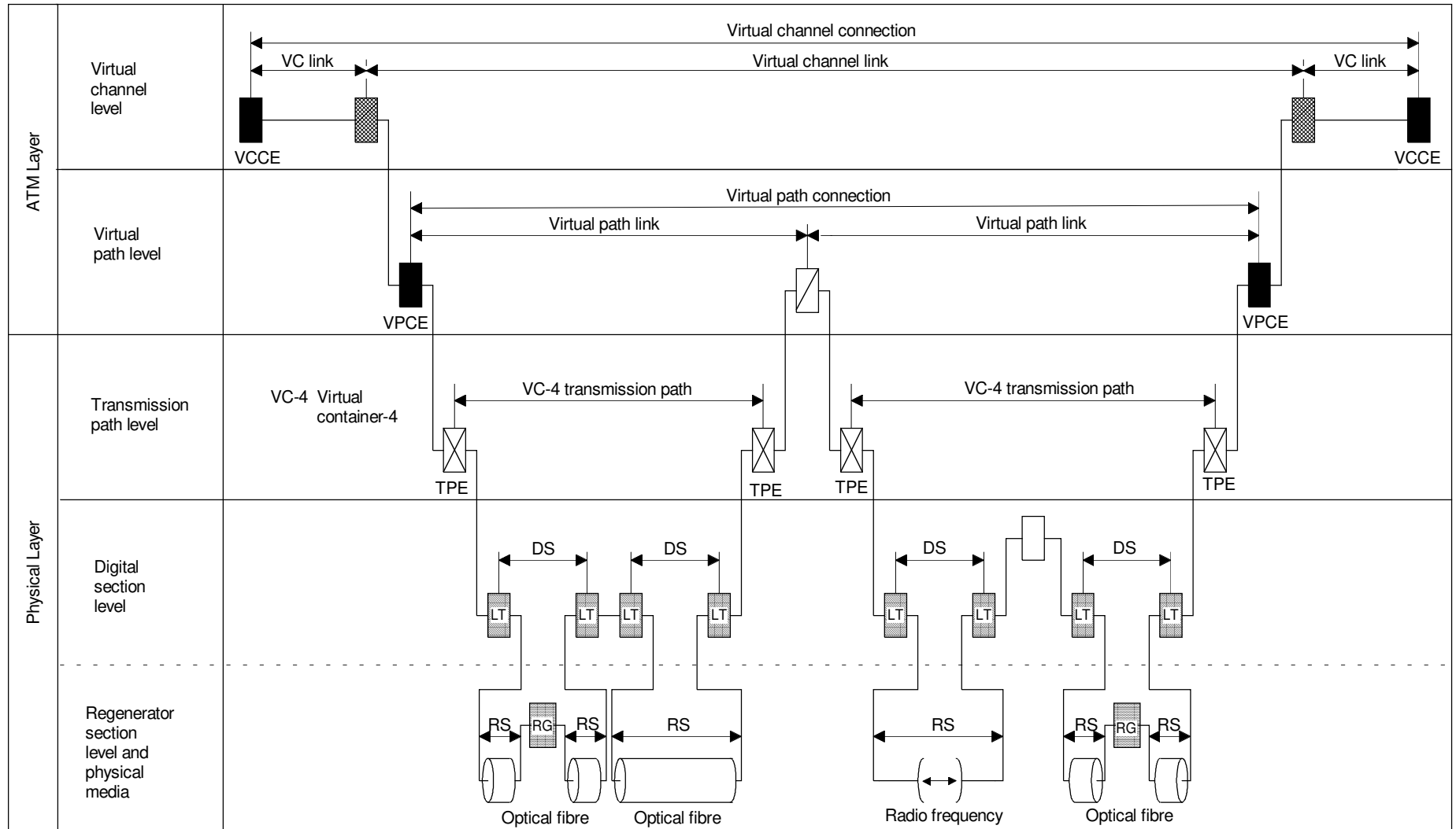
VCCE/VPCE Virtual channel connection endpoint Virtual path connection endpoint ATM switch (VC switch) ATM cross-connect (VP cross-connect) SDH cross connect TPE transmission path endpoint Regenerator Line termination DS Digital section RS Regenerator section
