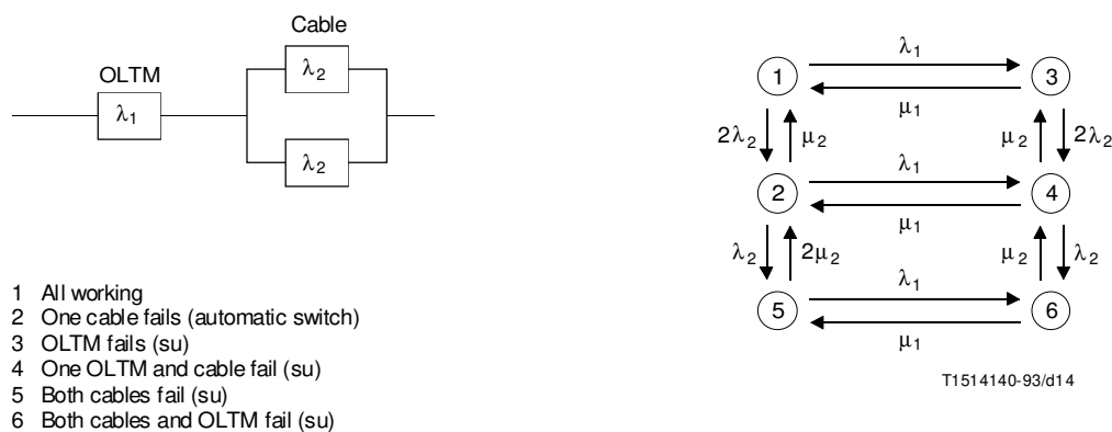
FIGURE C.5/G.911 Connection with cable redundancy and its Markov model
