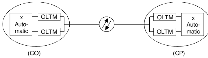
c) Connection with terminal equipment redundancy and automatic switchover
