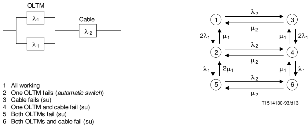
FIGURE C.4/G.911 Connection with terminal equipment redundancy and automatic switchover and its Markov model
