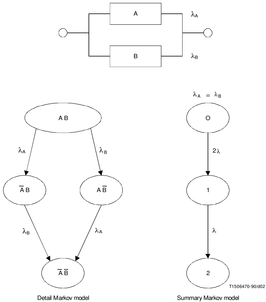
FIGURE 2/G.911 Examples of reliability block diagrams
