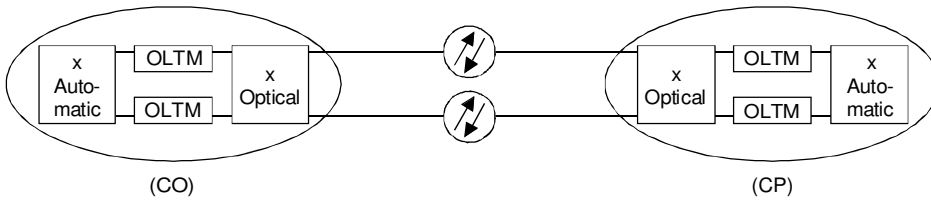
e1) Connection with terminal equipment and cable redundancy and automatic switchover
