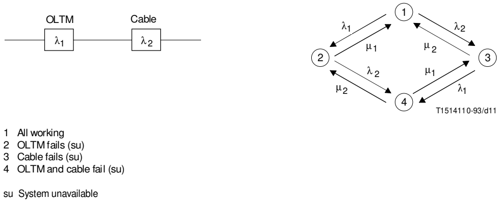
FIGURE C.2/G.911 No redundancy and its Markov model
