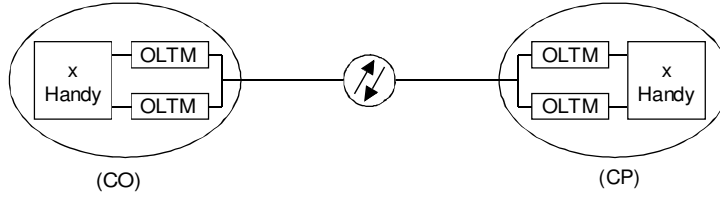
b) Connection with terminal equipment redundancy and manual switchover
