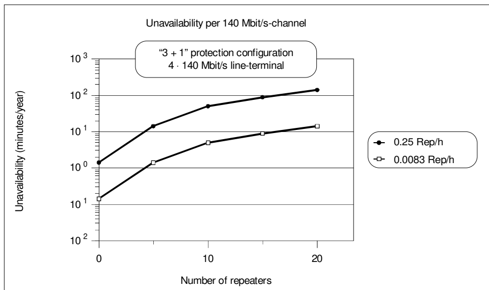
FIGURE B.3/G.911 Unavailability for 140 Mbit/s-channel
