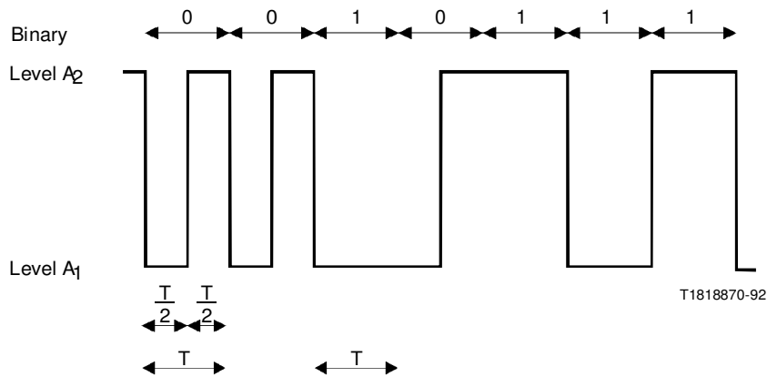
FIGURE 18/G.703
