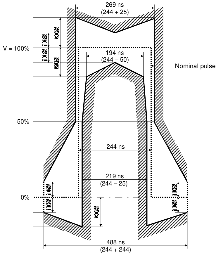
FIGURE 15/G.703
