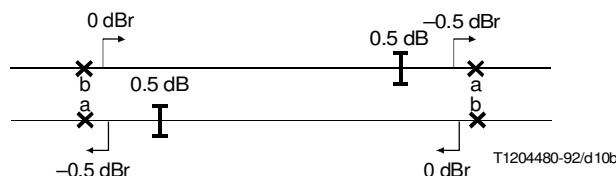
e) Type 5 circuit – All analogue circuit with analogue switching at both ends
