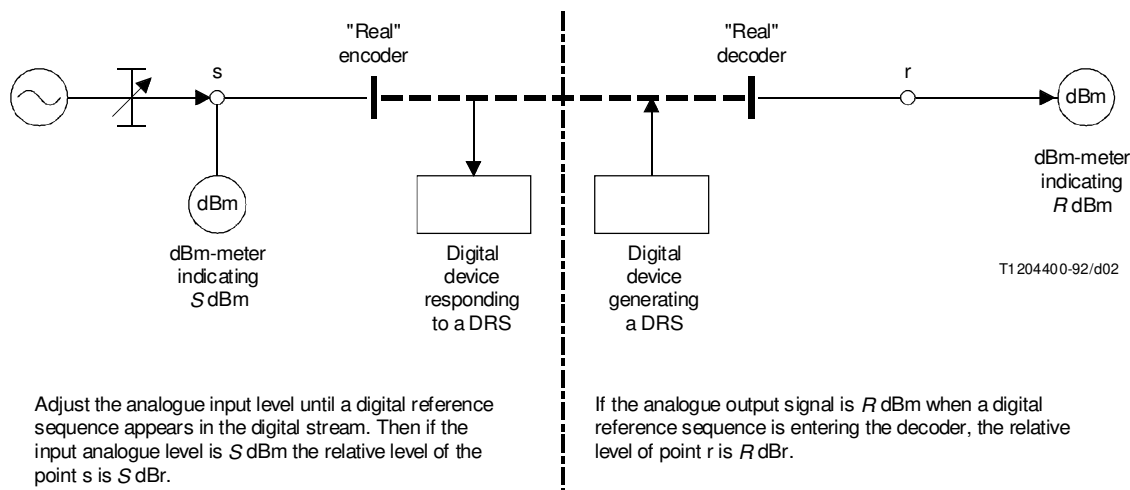
FIGURE 2/G.101
