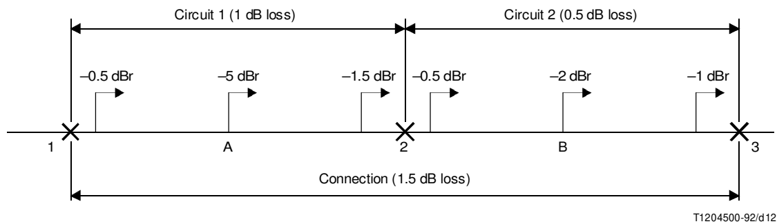
FIGURE A.2/G.101
