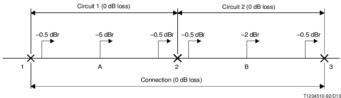
FIGURE A.3/G.101
