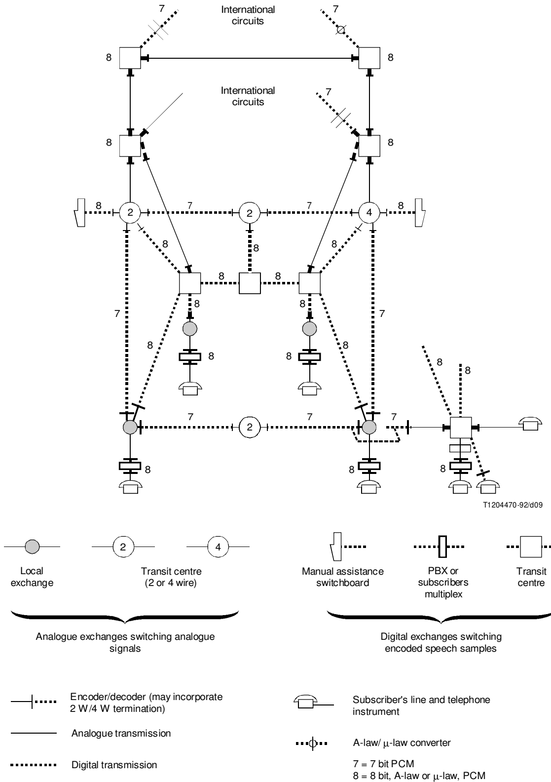
FIGURE 9/G.101
