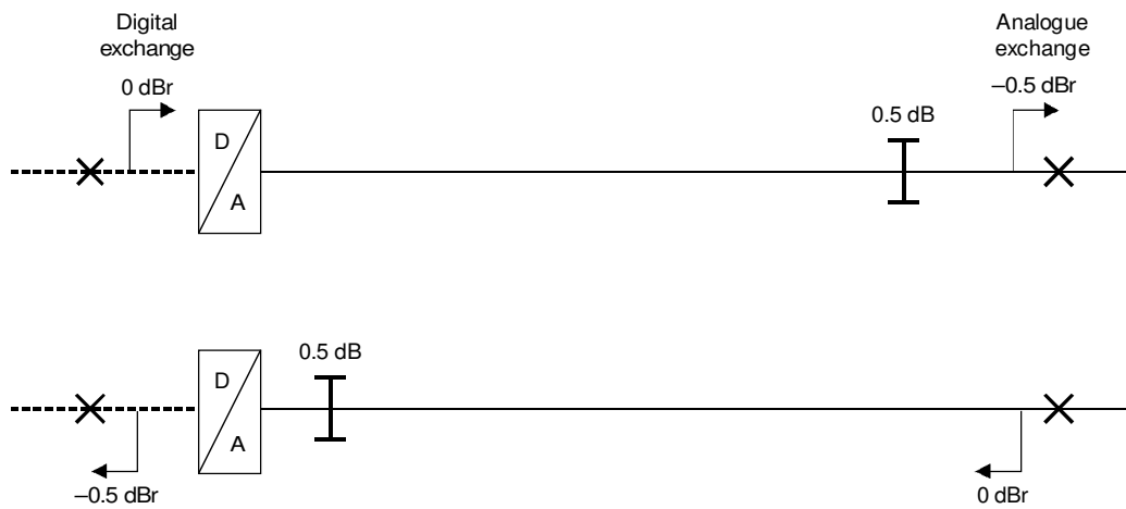
FIGURE A.4/G.101
