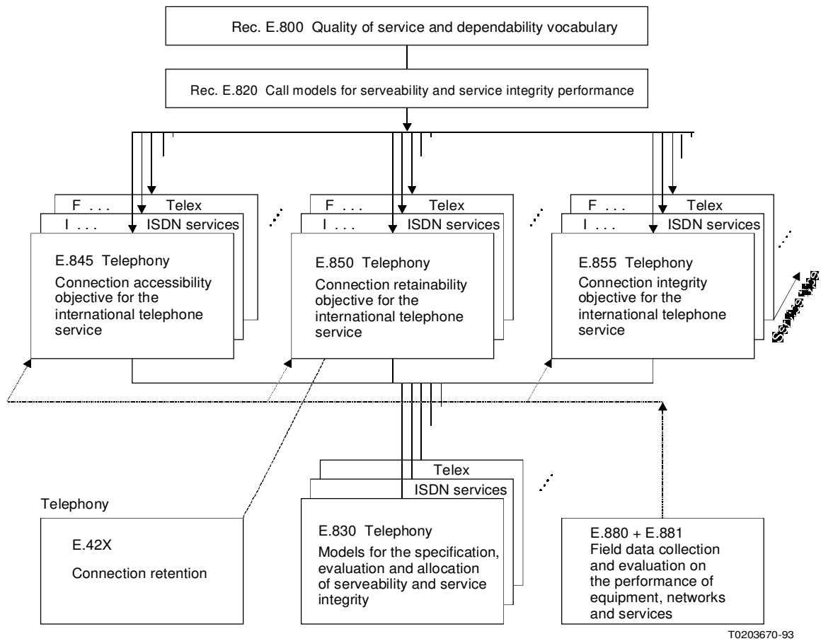
FIGURE 1/E.810 Relationship among serviceability and service integrity recommendations
