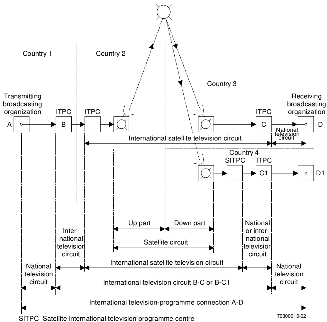
FIGURE 2/D.4 Example of an international television-programme connection involving a satellite circuit
