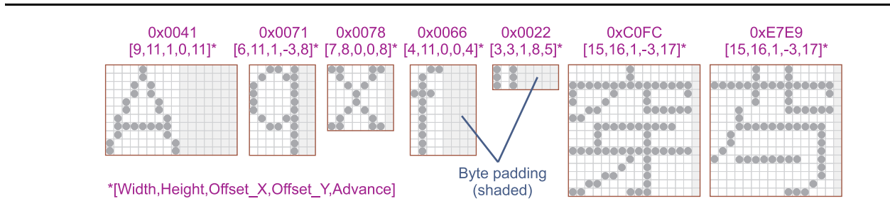
Figure 87. Proportional Font Parameters and Byte Padding
