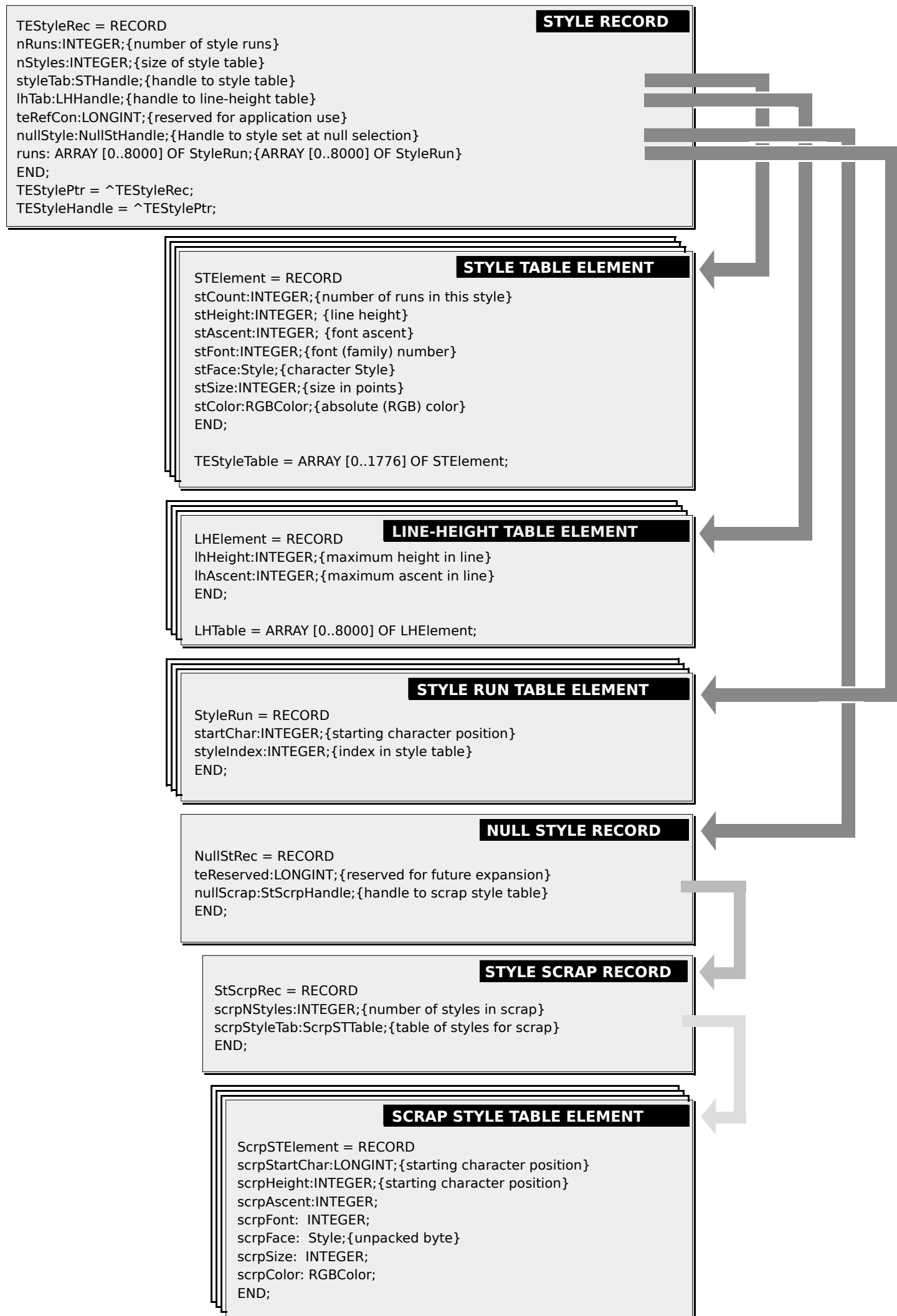
FIG 6 - THE STYLE RECORD AND SUBSIDIARY DATA STRUCTURES
