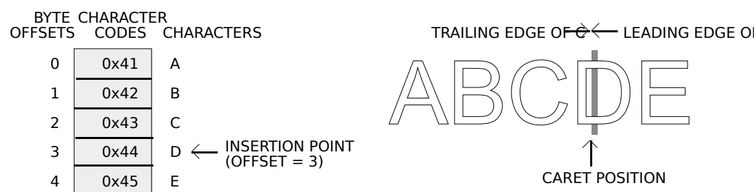
FIG 3 - CARET POSITION AND INSERTION POINT
